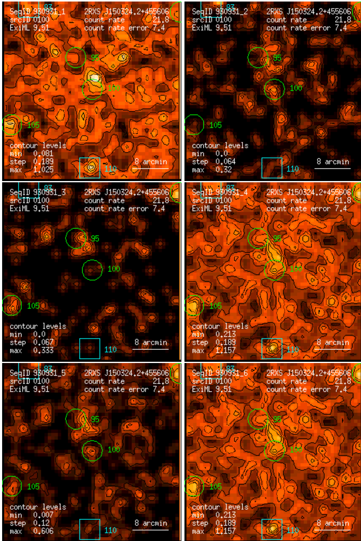
Figure 100: RASS 930931: detection 0100: band rate images, Gaussian filter: (1) PSPC channels 11 – 41, (2) 52 – 90, (3) 91 – 201, (4) 11 – 235, (5) 52 – 201, (6) 11 – 201. Broad band rates in counts/ks. Band rate contour levels in counts/ks/arcmin 2 .
