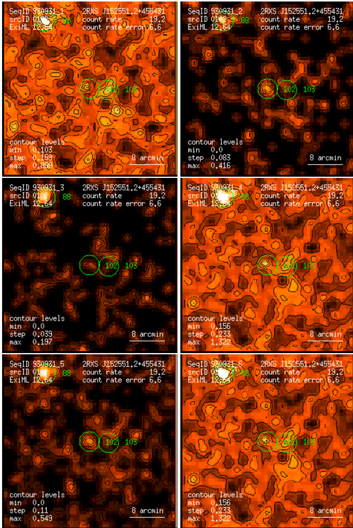
Figure 102: RASS 930931: detection 0102: band rate images, Gaussian filter: (1) PSPC channels 11 – 41, (2) 52 – 90, (3) 91 – 201, (4) 11 – 235, (5) 52 – 201, (6) 11 – 201. Broad band rates in counts/ks. Band rate contour levels in counts/ks/arcmin 2 .
