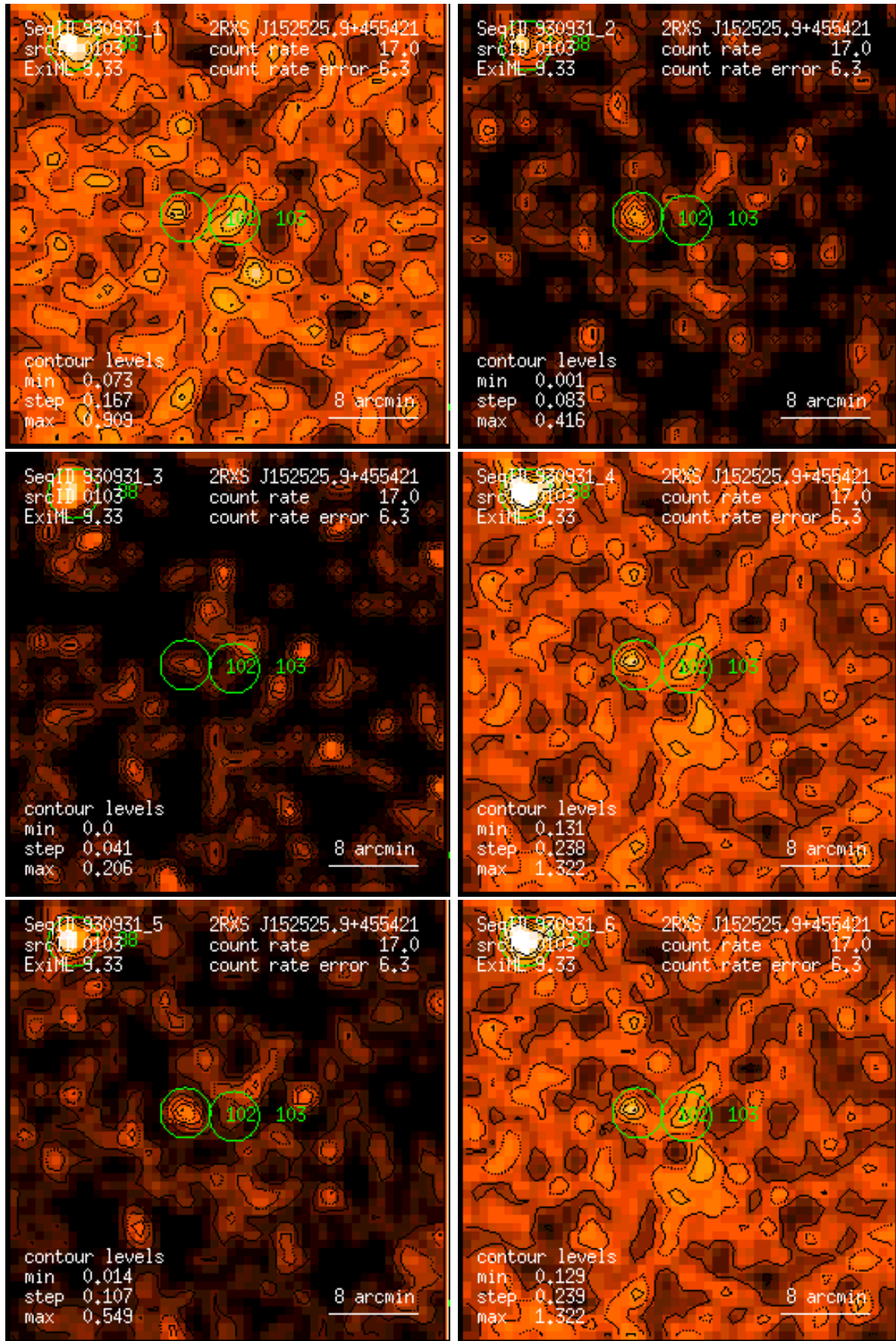
Figure 103: RASS 930931: detection 0103: band rate images, Gaussian filter: (1) PSPC channels 11 – 41, (2) 52 – 90, (3) 91 – 201, (4) 11 – 235, (5) 52 – 201, (6) 11 – 201. Broad band rates in counts/ks. Band rate contour levels in counts/ks/arcmin 2 .
