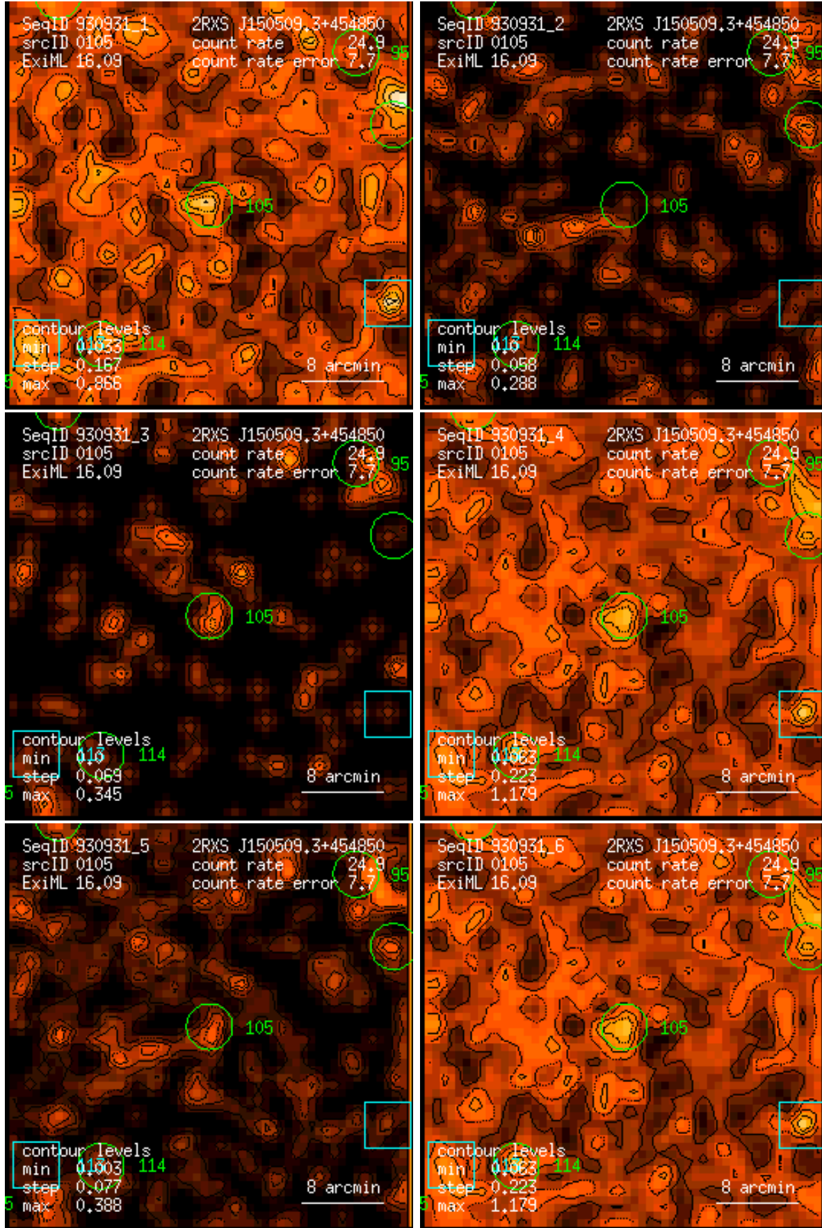
Figure 105: RASS 930931: detection 0105: band rate images, Gaussian filter: (1) PSPC channels 11 – 41, (2) 52 – 90, (3) 91 – 201, (4) 11 – 235, (5) 52 – 201, (6) 11 – 201. Broad band rates in counts/ks. Band rate contour levels in counts/ks/arcmin 2 .
