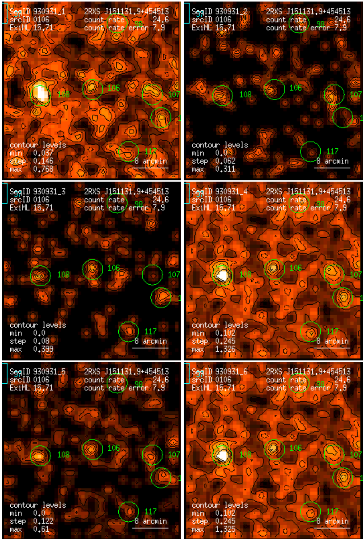
Figure 106: RASS 930931: detection 0106: band rate images, Gaussian filter: (1) PSPC channels 11 – 41, (2) 52 – 90, (3) 91 – 201, (4) 11 – 235, (5) 52 – 201, (6) 11 – 201. Broad band rates in counts/ks. Band rate contour levels in counts/ks/arcmin 2 .
