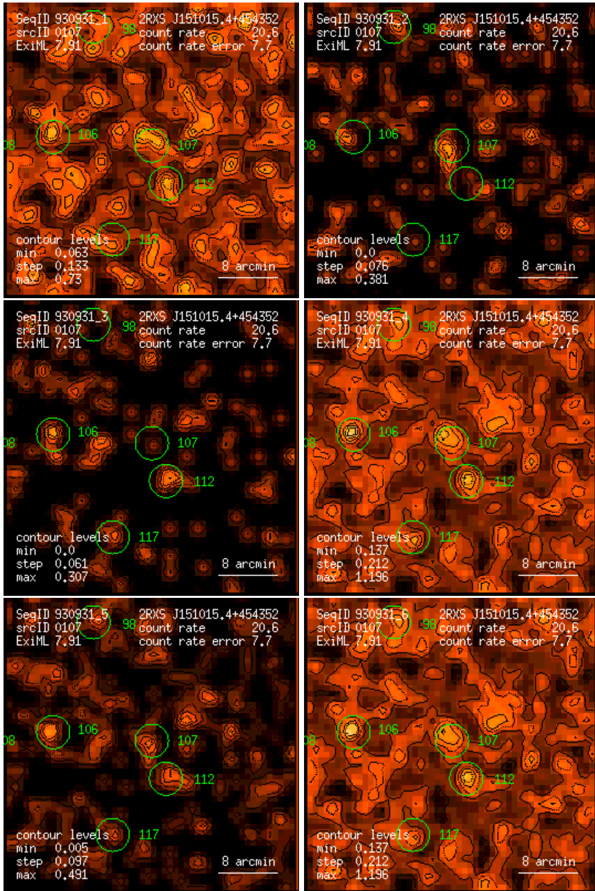
Figure 107: RASS 930931: detection 0107: band rate images, Gaussian filter: (1) PSPC channels 11 – 41, (2) 52 – 90, (3) 91 – 201, (4) 11 – 235, (5) 52 – 201, (6) 11 – 201. Broad band rates in counts/ks. Band rate contour levels in counts/ks/arcmin 2 .
