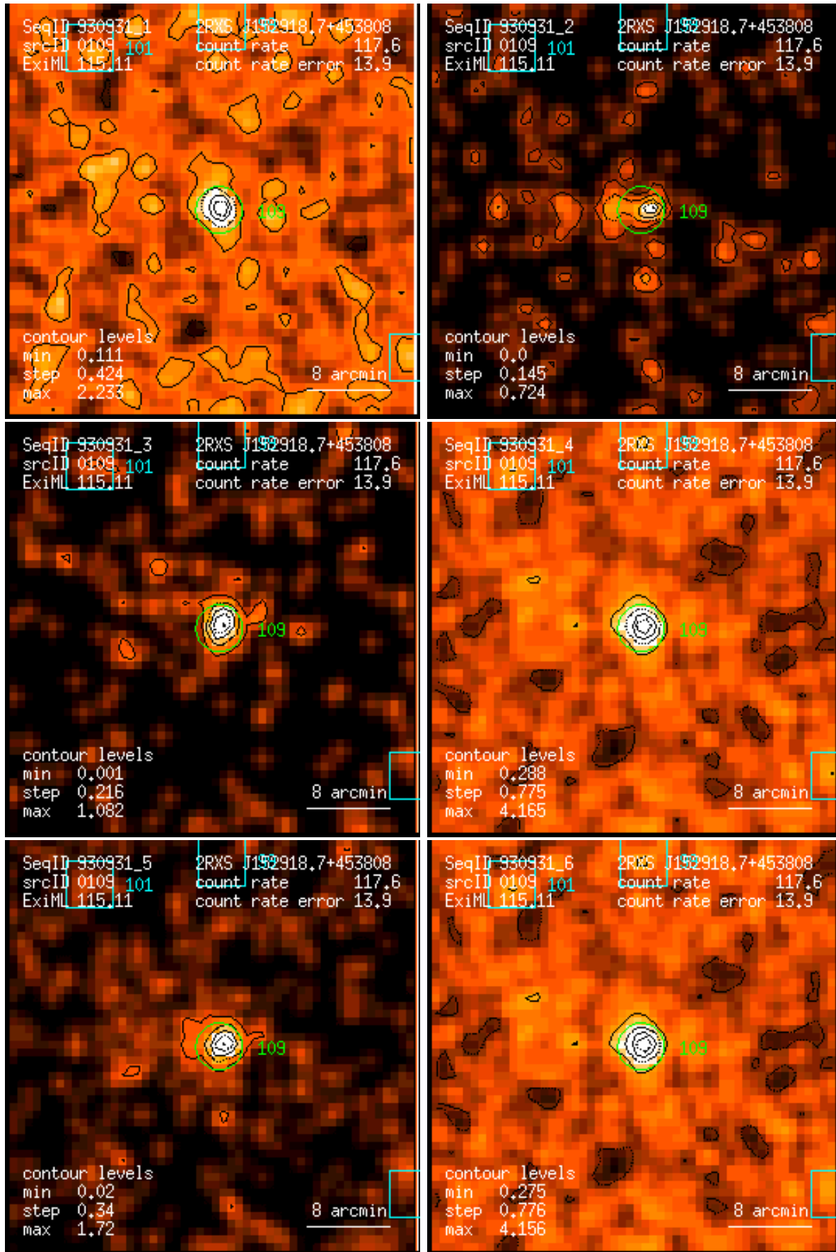
Figure 109: RASS 930931: detection 0109: band rate images, Gaussian filter: (1) PSPC channels 11 – 41, (2) 52 – 90, (3) 91 – 201, (4) 11 – 235, (5) 52 – 201, (6) 11 – 201. Broad band rates in counts/ks. Band rate contour levels in counts/ks/arcmin 2 .
