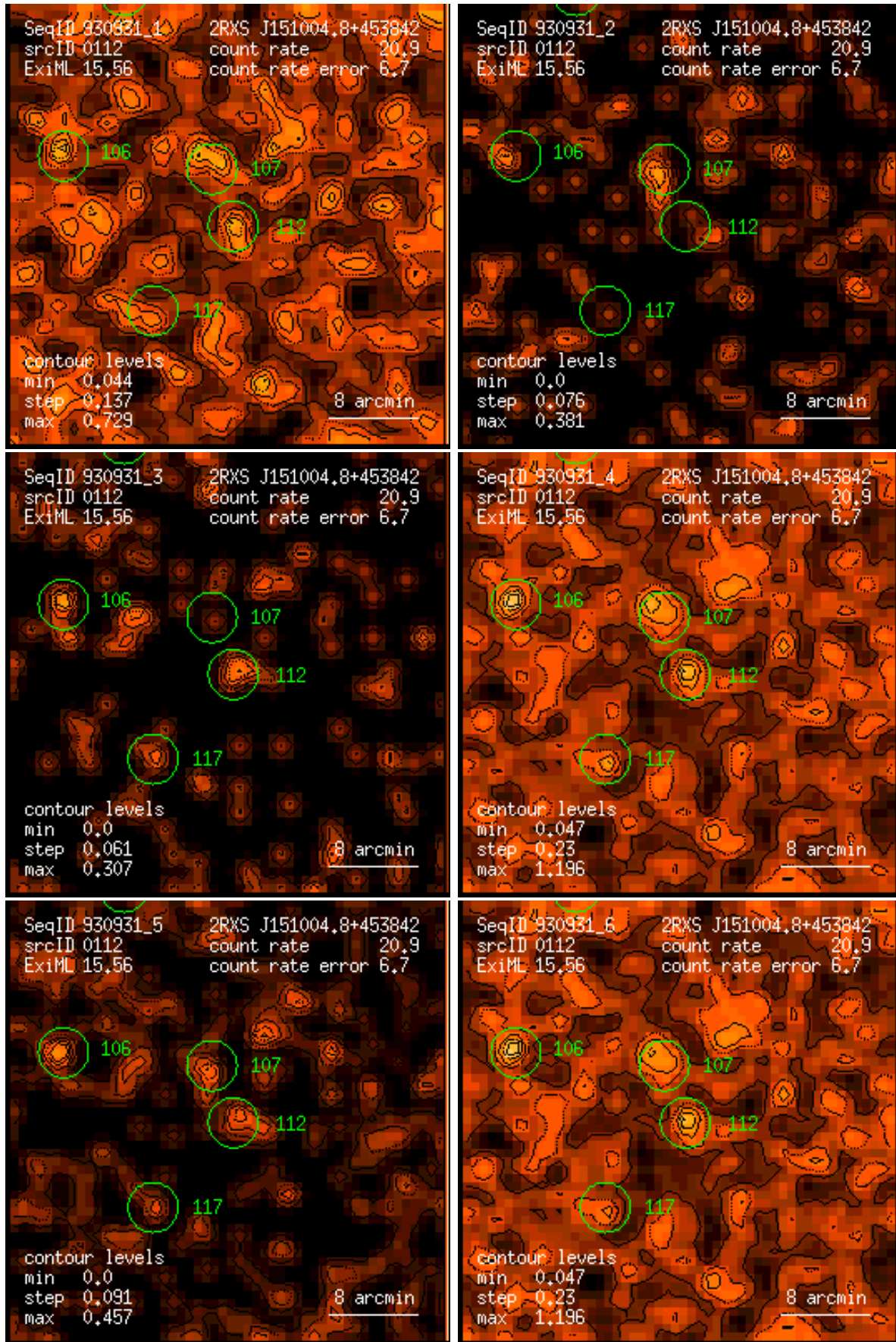
Figure 112: RASS 930931: detection 0112: band rate images, Gaussian filter: (1) PSPC channels 11 – 41, (2) 52 – 90, (3) 91 – 201, (4) 11 – 235, (5) 52 – 201, (6) 11 – 201. Broad band rates in counts/ks. Band rate contour levels in counts/ks/arcmin 2 .
