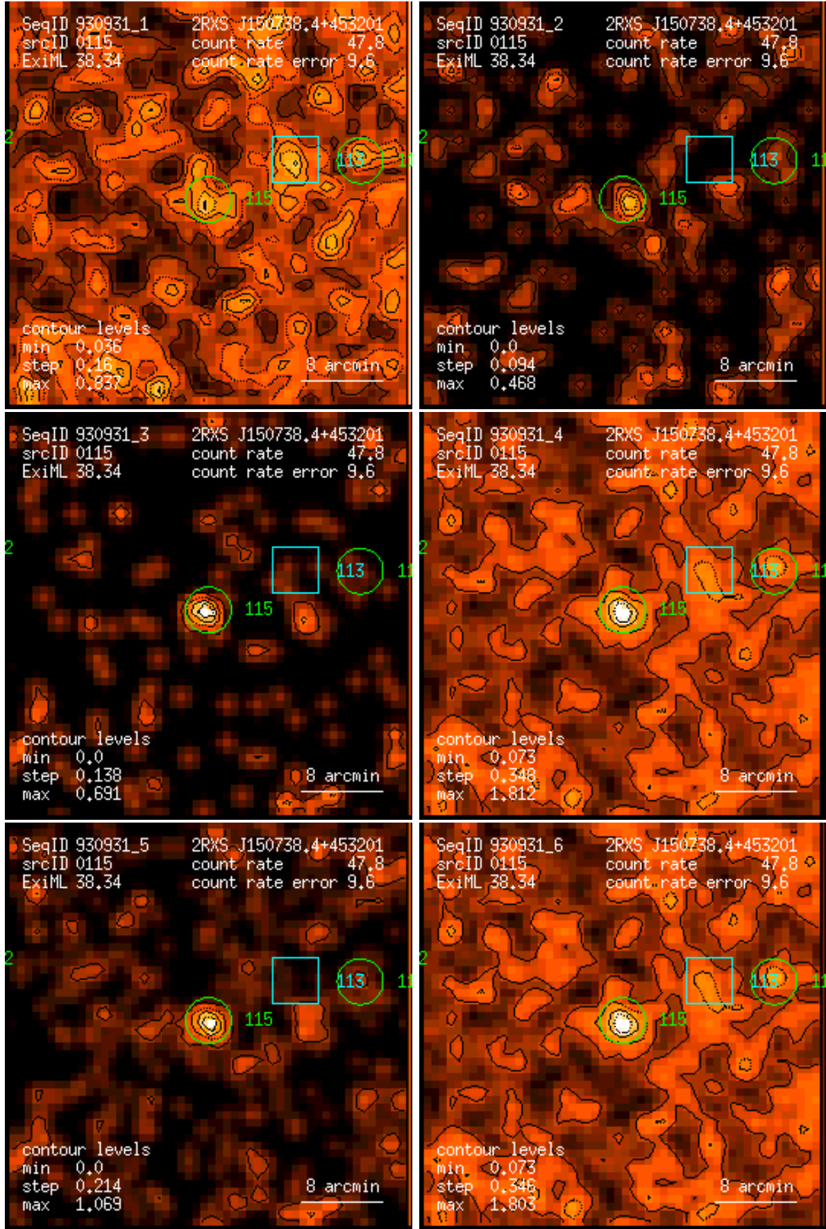
Figure 115: RASS 930931: detection 0115: band rate images, Gaussian filter: (1) PSPC channels 11 – 41, (2) 52 – 90, (3) 91 – 201, (4) 11 – 235, (5) 52 – 201, (6) 11 – 201. Broad band rates in counts/ks. Band rate contour levels in counts/ks/arcmin 2 .
