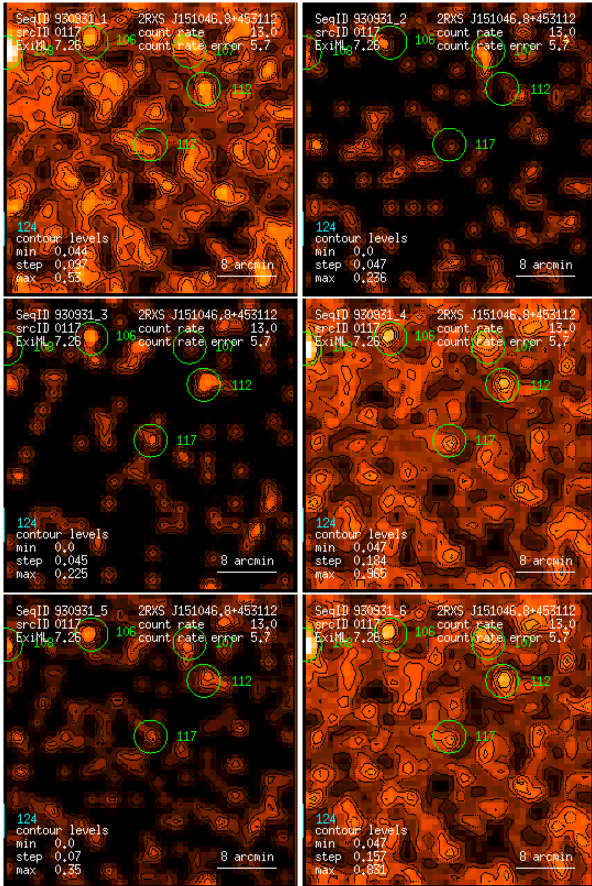
Figure 117: RASS 930931: detection 0117: band rate images, Gaussian filter: (1) PSPC channels 11 – 41, (2) 52 – 90, (3) 91 – 201, (4) 11 – 235, (5) 52 – 201, (6) 11 – 201. Broad band rates in counts/ks. Band rate contour levels in counts/ks/arcmin 2 .
