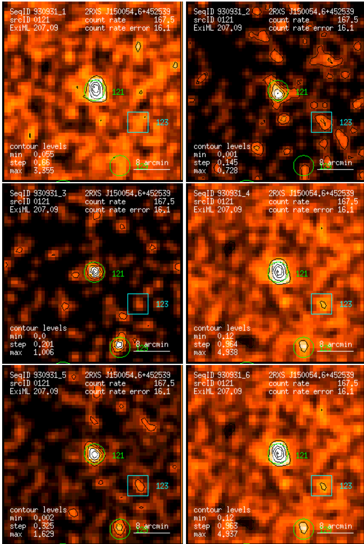
Figure 121: RASS 930931: detection 0121: band rate images, Gaussian filter: (1) PSPC channels 11 – 41, (2) 52 – 90, (3) 91 – 201, (4) 11 – 235, (5) 52 – 201, (6) 11 – 201. Broad band rates in counts/ks. Band rate contour levels in counts/ks/arcmin 2 .
