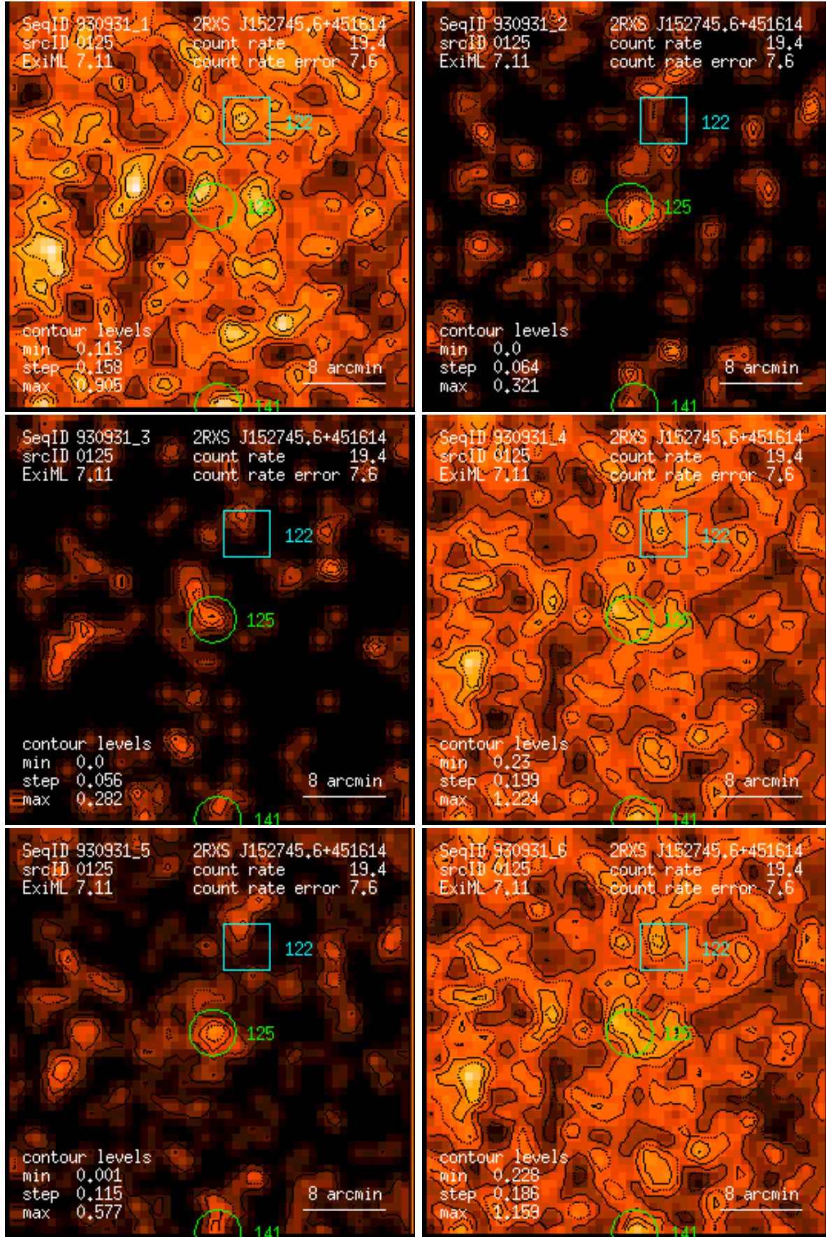
Figure 125: RASS 930931: detection 0125: band rate images, Gaussian filter: (1) PSPC channels 11 – 41, (2) 52 – 90, (3) 91 – 201, (4) 11 – 235, (5) 52 – 201, (6) 11 – 201. Broad band rates in counts/ks. Band rate contour levels in counts/ks/arcmin 2 .
