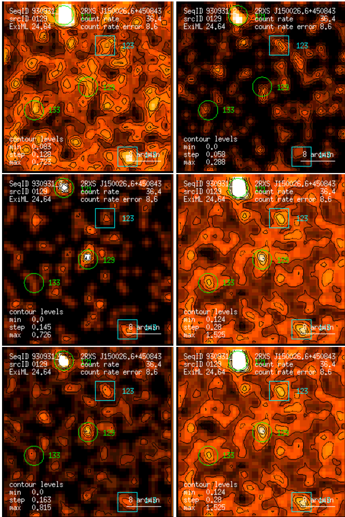
Figure 129: RASS 930931: detection 0129: band rate images, Gaussian filter: (1) PSPC channels 11 – 41, (2) 52 – 90, (3) 91 – 201, (4) 11 – 235, (5) 52 – 201, (6) 11 – 201. Broad band rates in counts/ks. Band rate contour levels in counts/ks/arcmin 2 .
