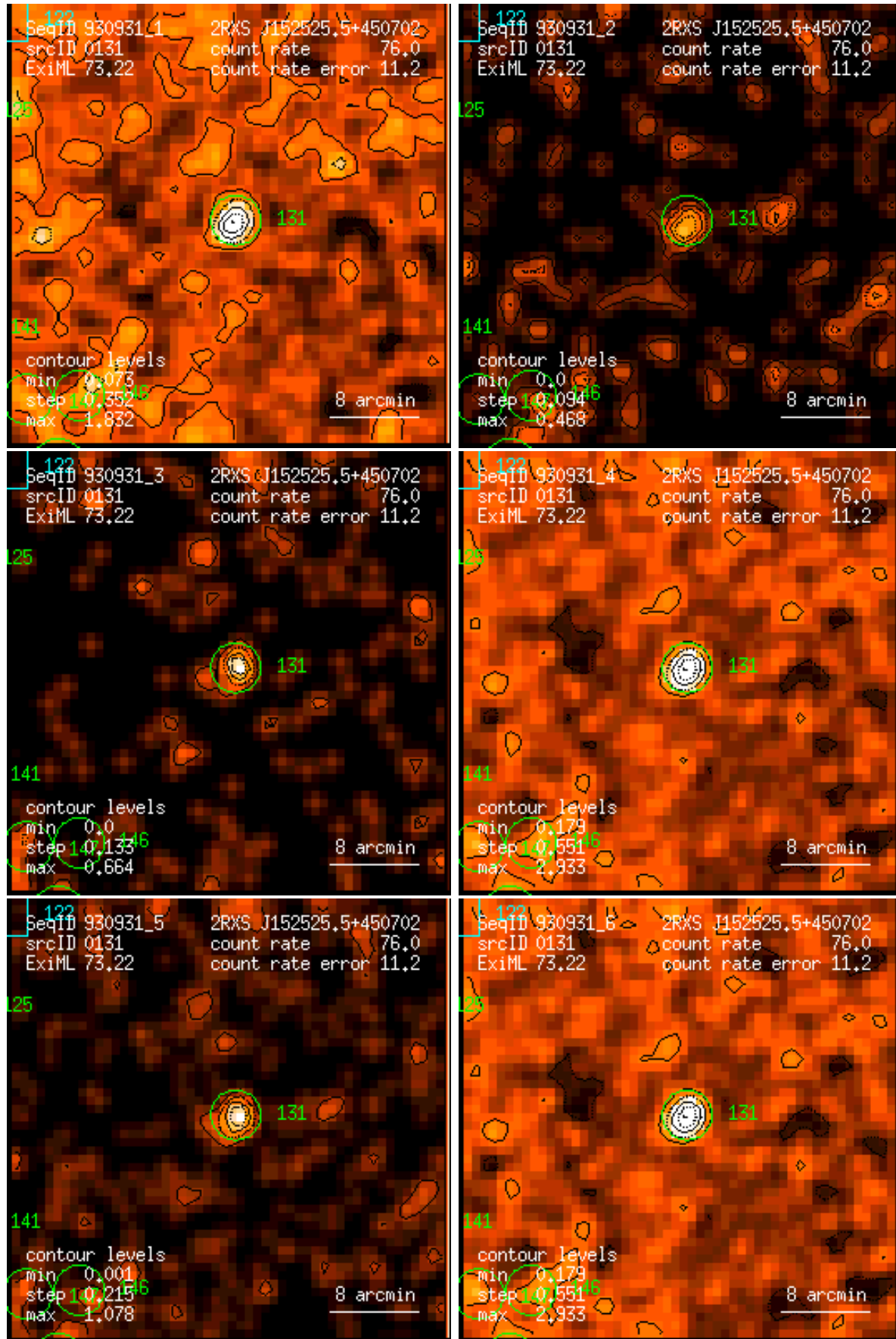
Figure 131: RASS 930931: detection 0131: band rate images, Gaussian filter: (1) PSPC channels 11 – 41, (2) 52 – 90, (3) 91 – 201, (4) 11 – 235, (5) 52 – 201, (6) 11 – 201. Broad band rates in counts/ks. Band rate contour levels in counts/ks/arcmin 2 .
