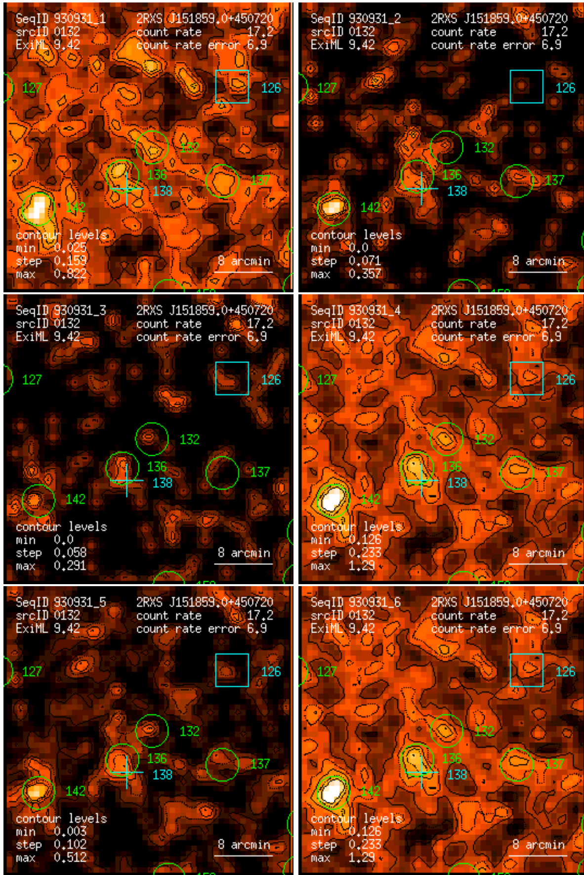
Figure 132: RASS 930931: detection 0132: band rate images, Gaussian filter: (1) PSPC channels 11 – 41, (2) 52 – 90, (3) 91 – 201, (4) 11 – 235, (5) 52 – 201, (6) 11 – 201. Broad band rates in counts/ks. Band rate contour levels in counts/ks/arcmin 2 .
