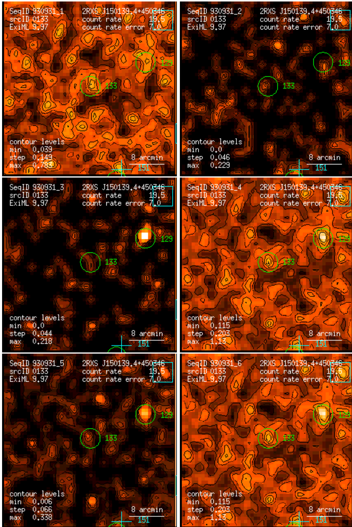
Figure 133: RASS 930931: detection 0133: band rate images, Gaussian filter: (1) PSPC channels 11 – 41, (2) 52 – 90, (3) 91 – 201, (4) 11 – 235, (5) 52 – 201, (6) 11 – 201. Broad band rates in counts/ks. Band rate contour levels in counts/ks/arcmin 2 .
