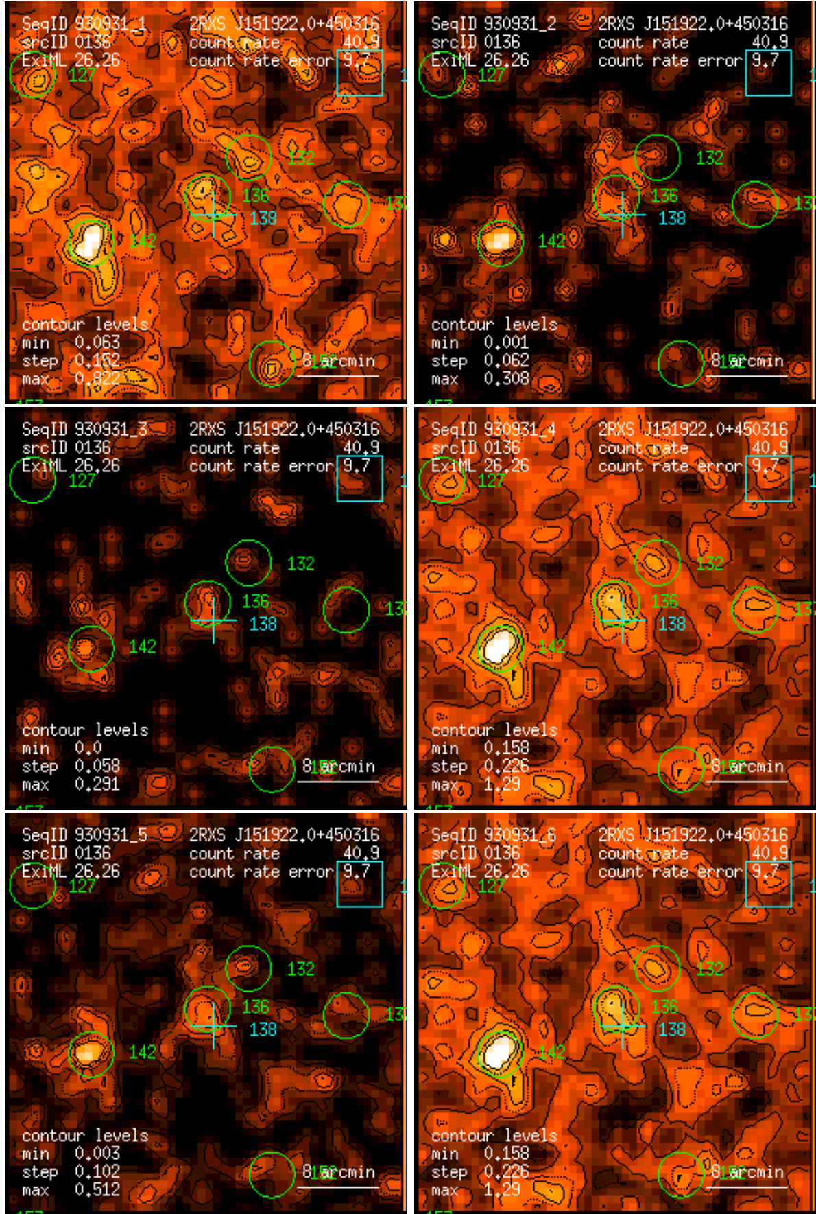
Figure 136: RASS 930931: detection 0136: band rate images, Gaussian filter: (1) PSPC channels 11 – 41, (2) 52 – 90, (3) 91 – 201, (4) 11 – 235, (5) 52 – 201, (6) 11 – 201. Broad band rates in counts/ks. Band rate contour levels in counts/ks/arcmin 2 .
