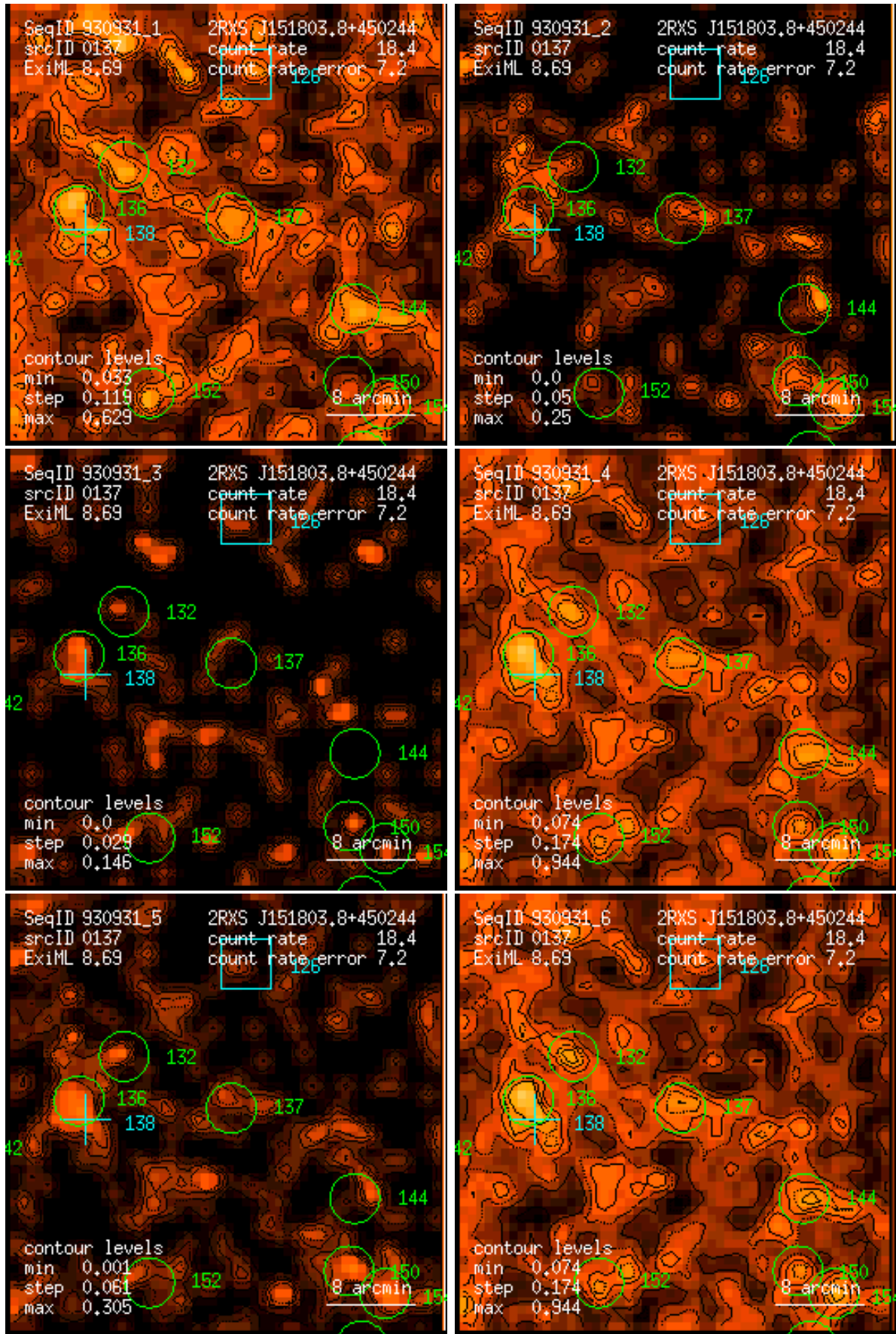
Figure 137: RASS 930931: detection 0137: band rate images, Gaussian filter: (1) PSPC channels 11 – 41, (2) 52 – 90, (3) 91 – 201, (4) 11 – 235, (5) 52 – 201, (6) 11 – 201. Broad band rates in counts/ks. Band rate contour levels in counts/ks/arcmin 2 .
