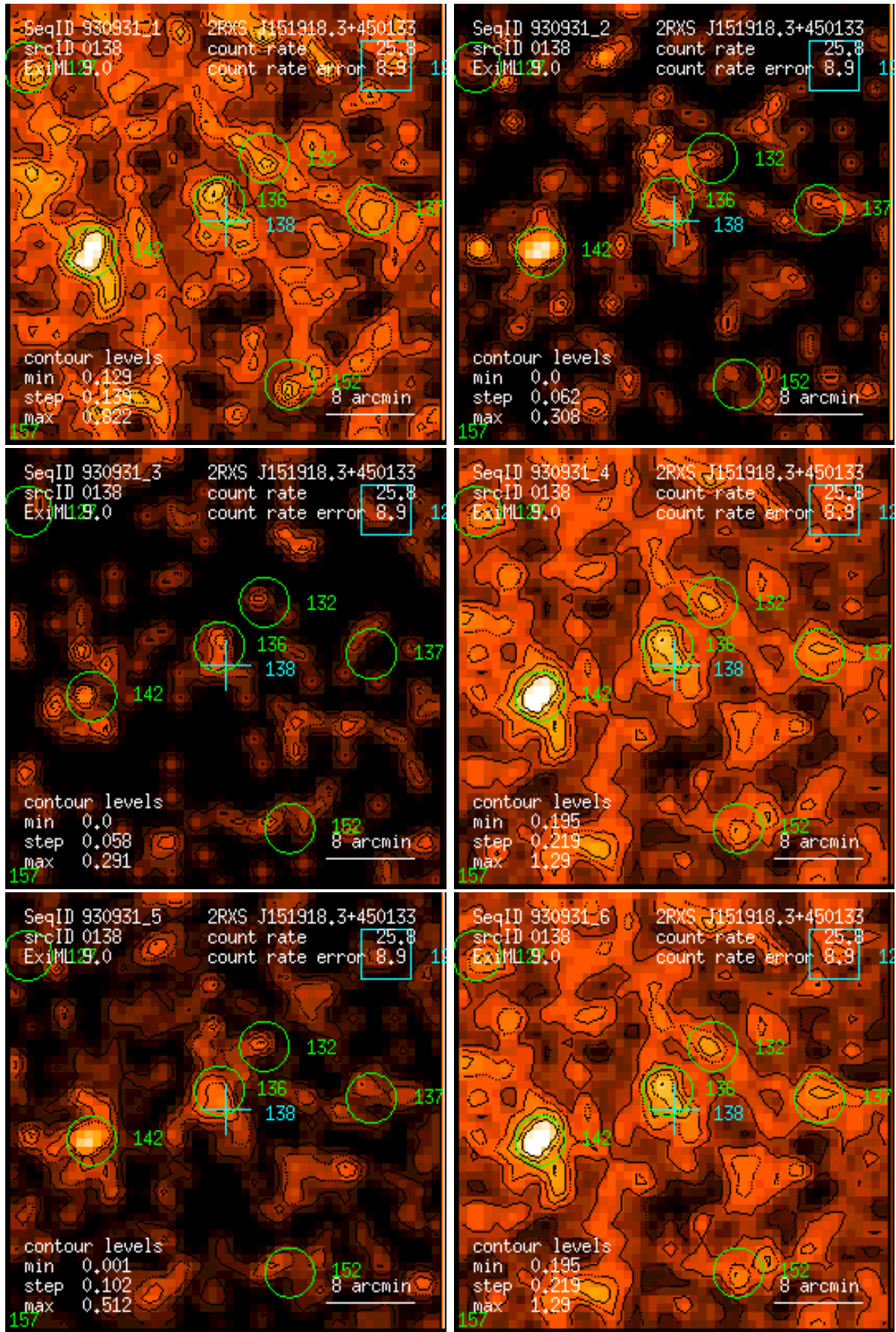
Figure 138: RASS 930931: detection 0138: band rate images, Gaussian filter: (1) PSPC channels 11 – 41, (2) 52 – 90, (3) 91 – 201, (4) 11 – 235, (5) 52 – 201, (6) 11 – 201. Broad band rates in counts/ks. Band rate contour levels in counts/ks/arcmin 2 .
