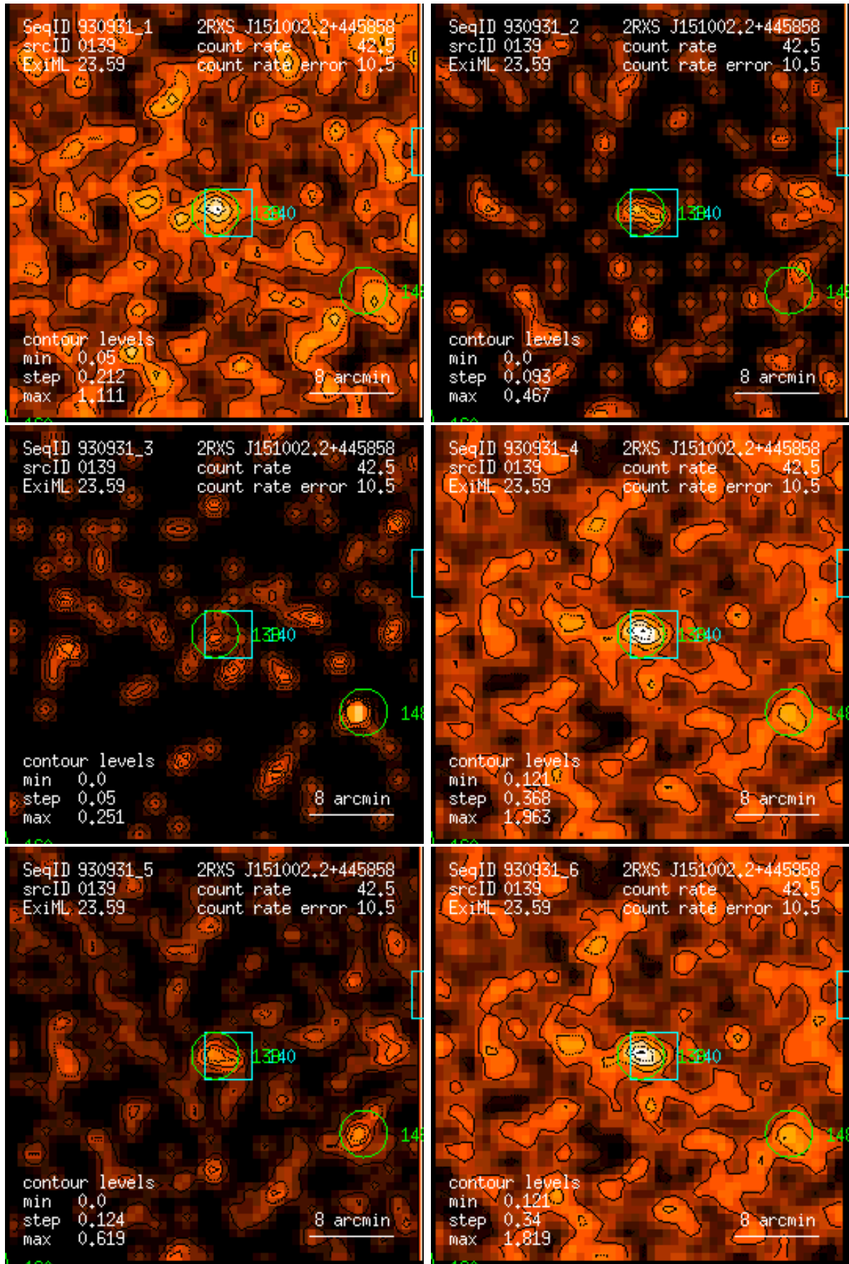
Figure 139: RASS 930931: detection 0139: band rate images, Gaussian filter: (1) PSPC channels 11 – 41, (2) 52 – 90, (3) 91 – 201, (4) 11 – 235, (5) 52 – 201, (6) 11 – 201. Broad band rates in counts/ks. Band rate contour levels in counts/ks/arcmin 2 .
