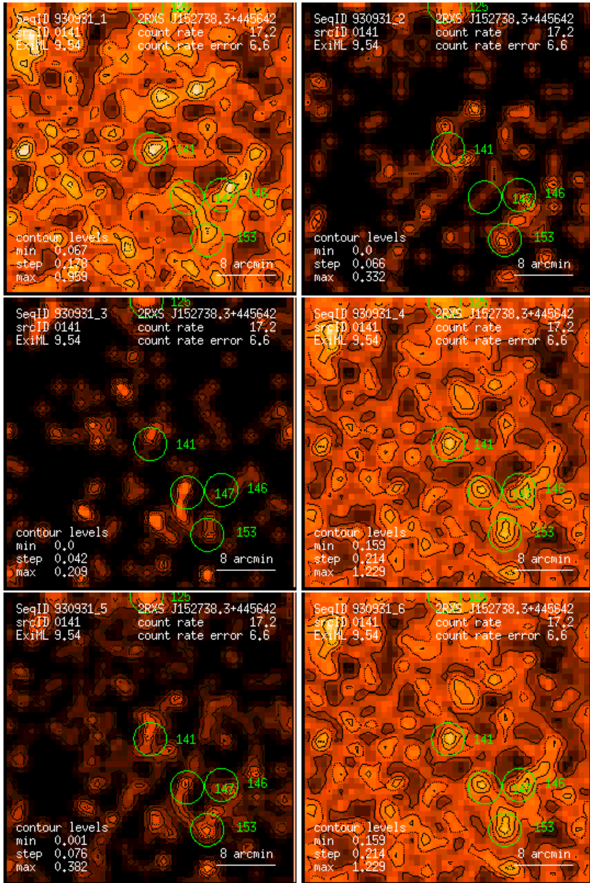
Figure 141: RASS 930931: detection 0141: band rate images, Gaussian filter: (1) PSPC channels 11 – 41, (2) 52 – 90, (3) 91 – 201, (4) 11 – 235, (5) 52 – 201, (6) 11 – 201. Broad band rates in counts/ks. Band rate contour levels in counts/ks/arcmin 2 .
