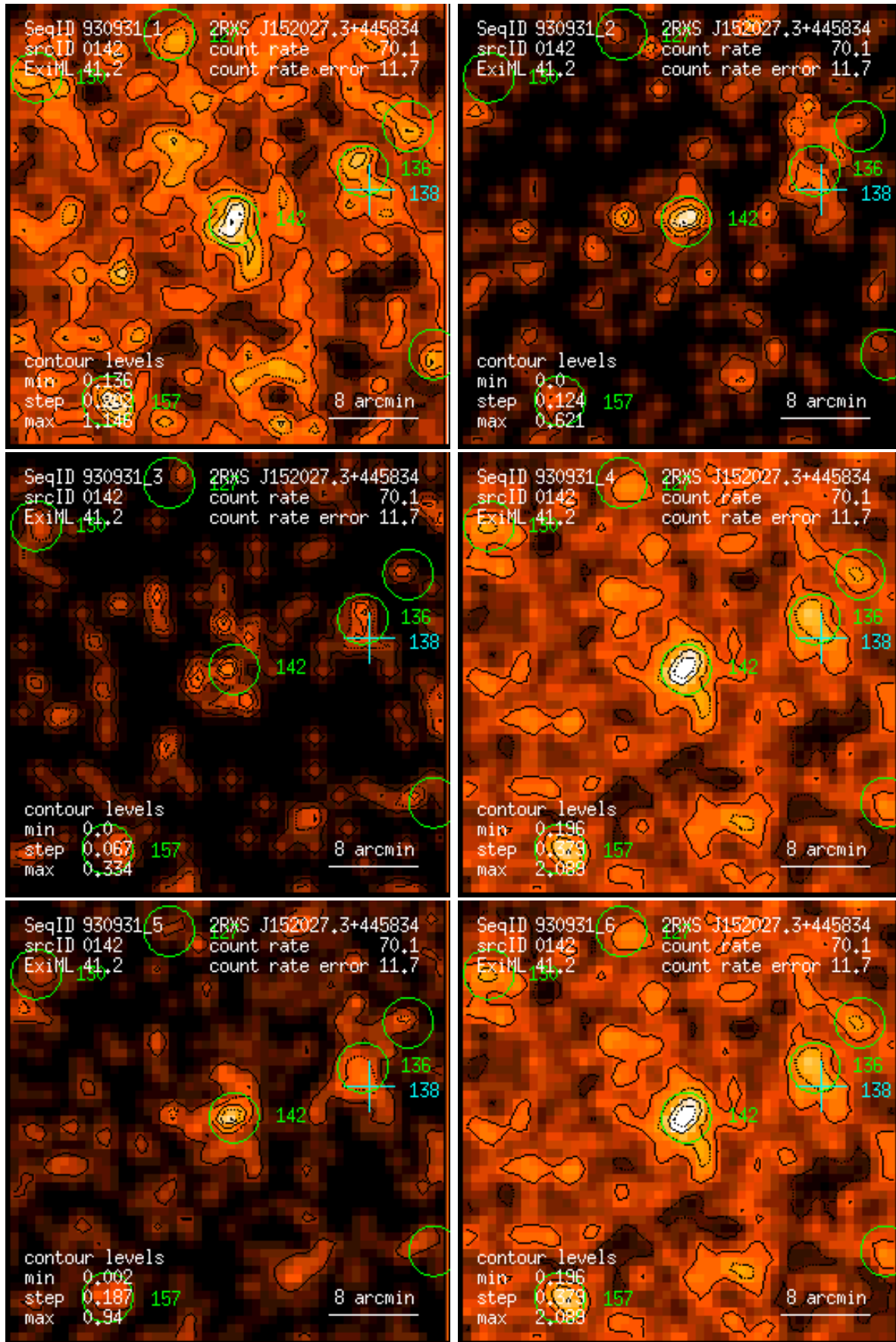
Figure 142: RASS 930931: detection 0142: band rate images, Gaussian filter: (1) PSPC channels 11 – 41, (2) 52 – 90, (3) 91 – 201, (4) 11 – 235, (5) 52 – 201, (6) 11 – 201. Broad band rates in counts/ks. Band rate contour levels in counts/ks/arcmin 2 .
