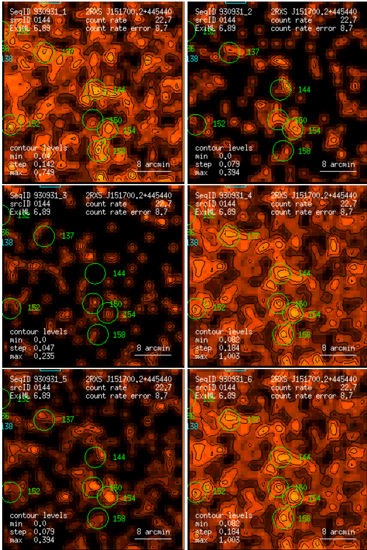
Figure 144: RASS 930931: detection 0144: band rate images, Gaussian filter: (1) PSPC channels 11 – 41, (2) 52 – 90, (3) 91 – 201, (4) 11 – 235, (5) 52 – 201, (6) 11 – 201. Broad band rates in counts/ks. Band rate contour levels in counts/ks/arcmin 2 .
