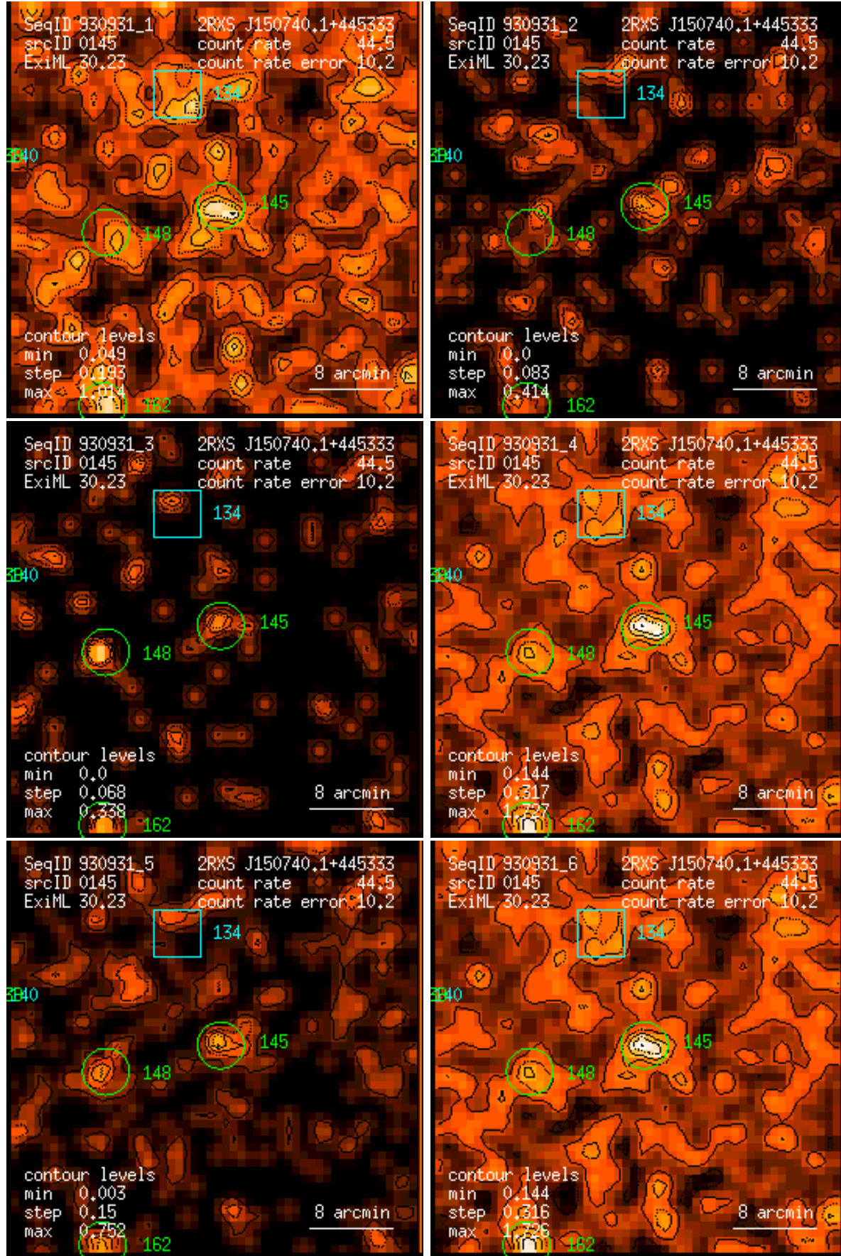
Figure 145: RASS 930931: detection 0145: band rate images, Gaussian filter: (1) PSPC channels 11 – 41, (2) 52 – 90, (3) 91 – 201, (4) 11 – 235, (5) 52 – 201, (6) 11 – 201. Broad band rates in counts/ks. Band rate contour levels in counts/ks/arcmin 2 .
