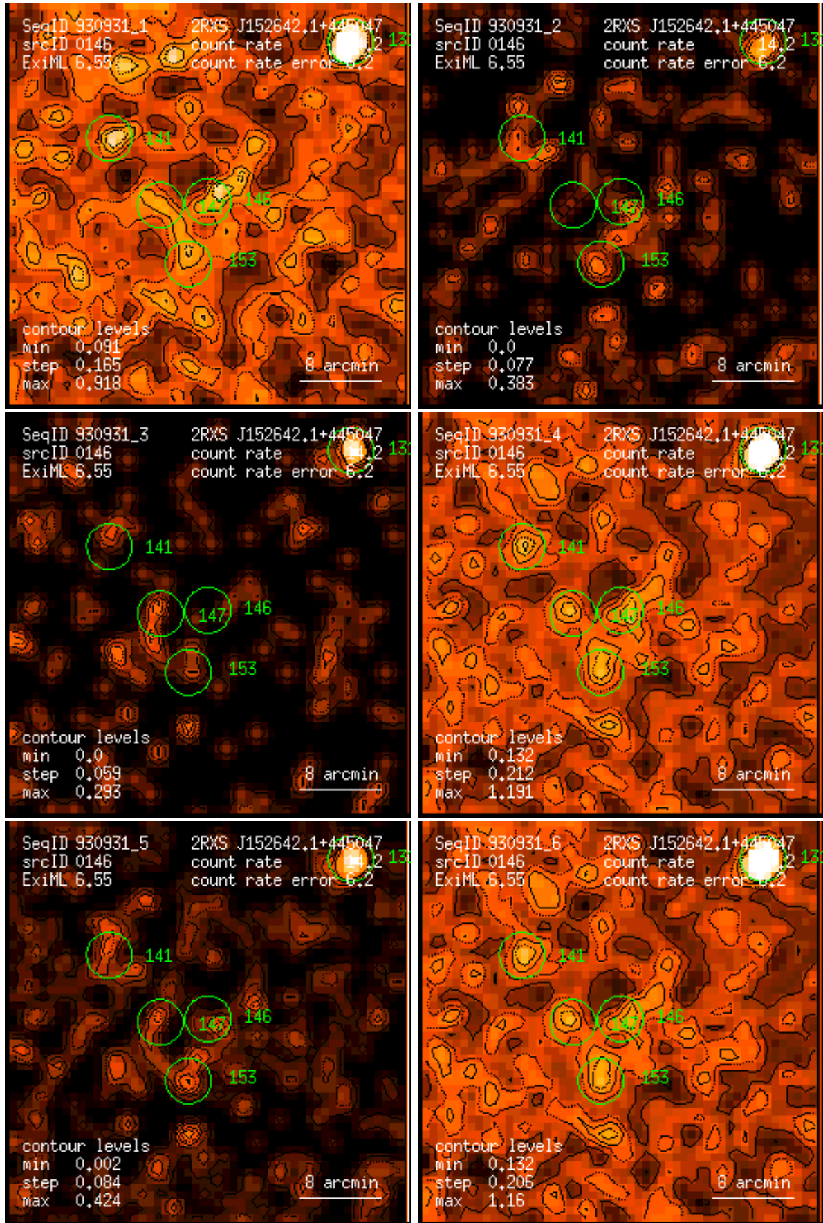
Figure 146: RASS 930931: detection 0146: band rate images, Gaussian filter: (1) PSPC channels 11 – 41, (2) 52 – 90, (3) 91 – 201, (4) 11 – 235, (5) 52 – 201, (6) 11 – 201. Broad band rates in counts/ks. Band rate contour levels in counts/ks/arcmin 2 .
