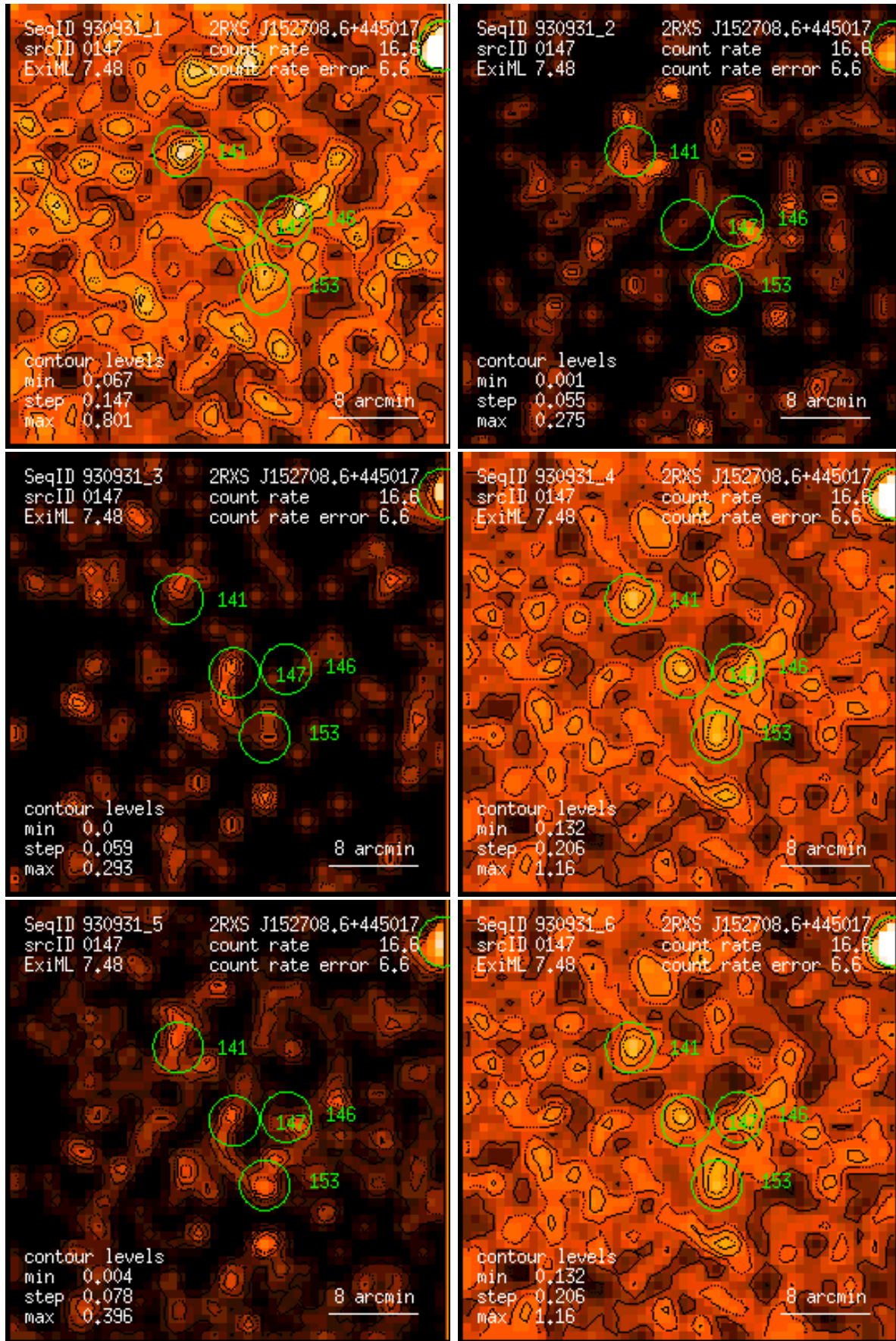
Figure 147: RASS 930931: detection 0147: band rate images, Gaussian filter: (1) PSPC channels 11 – 41, (2) 52 – 90, (3) 91 – 201, (4) 11 – 235, (5) 52 – 201, (6) 11 – 201. Broad band rates in counts/ks. Band rate contour levels in counts/ks/arcmin 2 .
