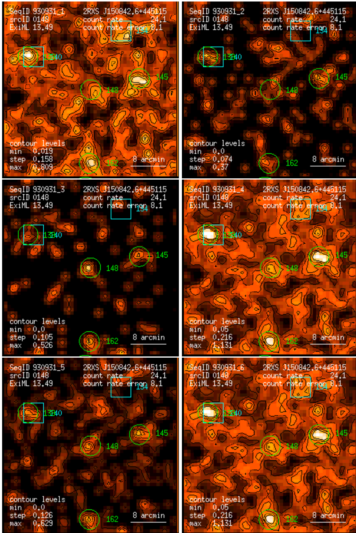
Figure 148: RASS 930931: detection 0148: band rate images, Gaussian filter: (1) PSPC channels 11 – 41, (2) 52 – 90, (3) 91 – 201, (4) 11 – 235, (5) 52 – 201, (6) 11 – 201. Broad band rates in counts/ks. Band rate contour levels in counts/ks/arcmin 2 .
