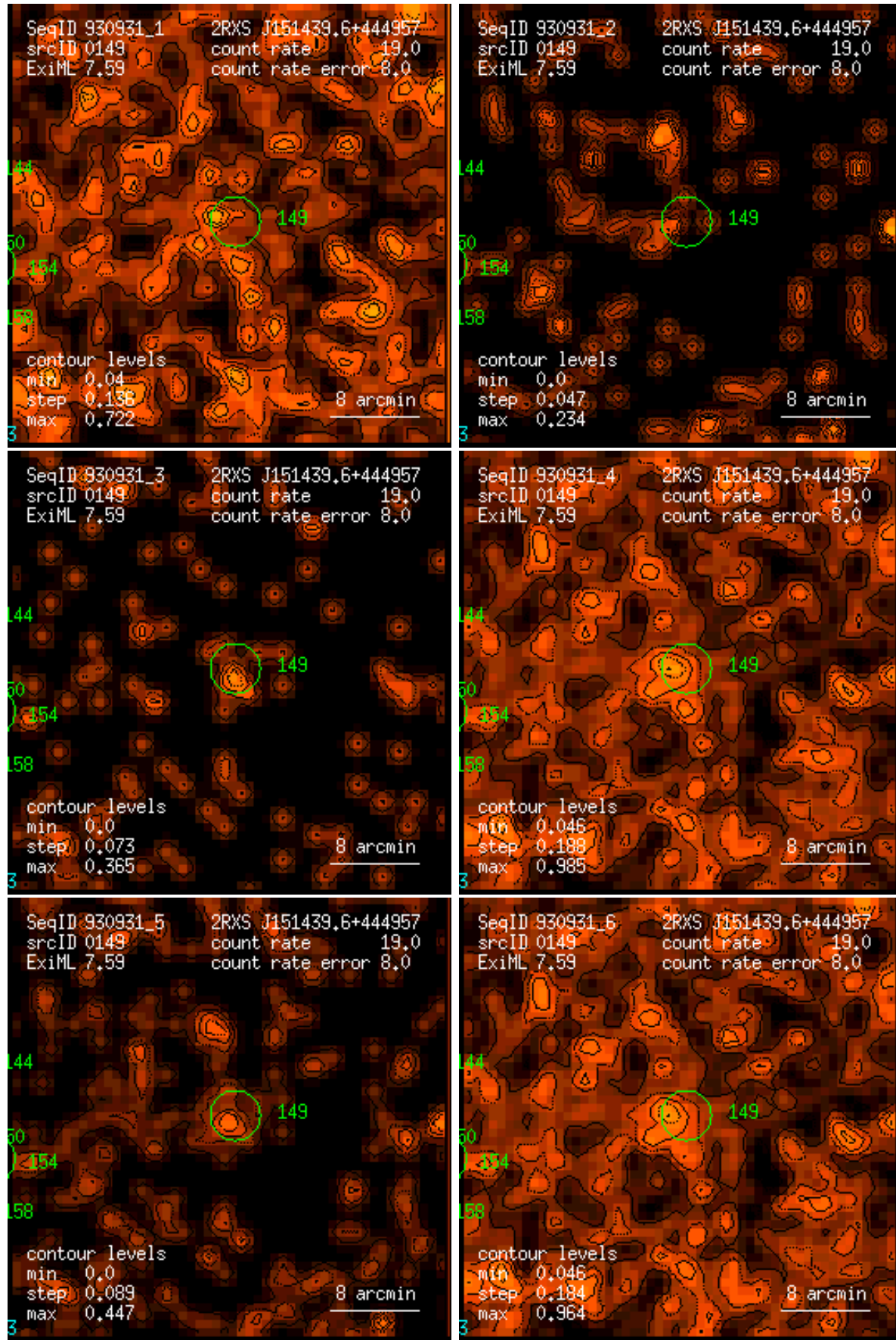
Figure 149: RASS 930931: detection 0149: band rate images, Gaussian filter: (1) PSPC channels 11 – 41, (2) 52 – 90, (3) 91 – 201, (4) 11 – 235, (5) 52 – 201, (6) 11 – 201. Broad band rates in counts/ks. Band rate contour levels in counts/ks/arcmin 2 .
