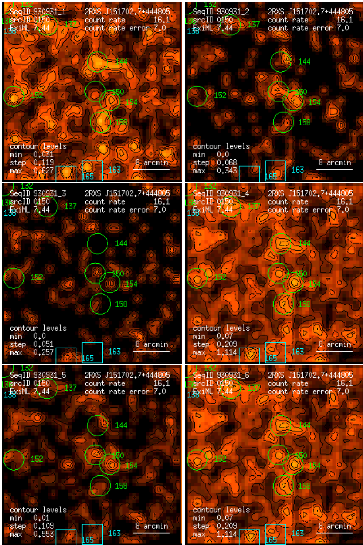
Figure 150: RASS 930931: detection 0150: band rate images, Gaussian filter: (1) PSPC channels 11 – 41, (2) 52 – 90, (3) 91 – 201, (4) 11 – 235, (5) 52 – 201, (6) 11 – 201. Broad band rates in counts/ks. Band rate contour levels in counts/ks/arcmin 2 .
