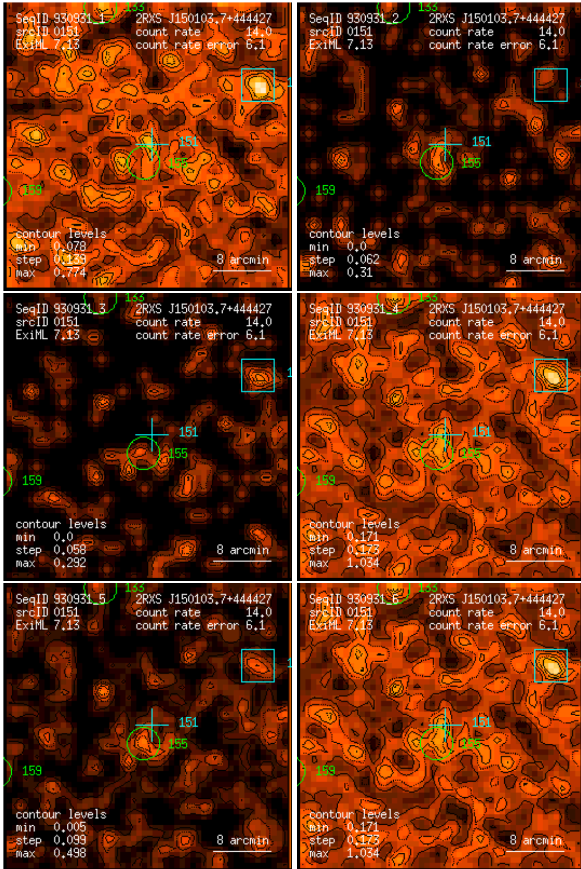
Figure 151: RASS 930931: detection 0151: band rate images, Gaussian filter: (1) PSPC channels 11 – 41, (2) 52 – 90, (3) 91 – 201, (4) 11 – 235, (5) 52 – 201, (6) 11 – 201. Broad band rates in counts/ks. Band rate contour levels in counts/ks/arcmin 2 .
