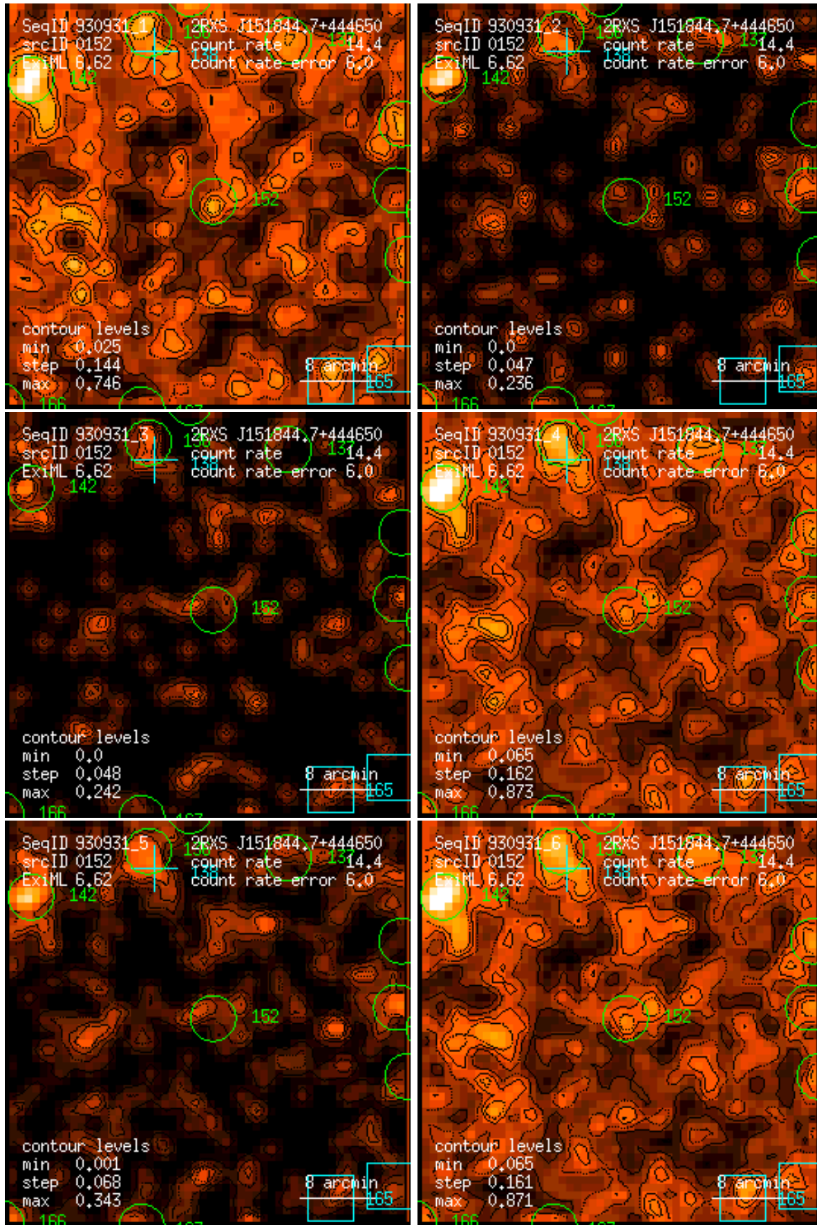
Figure 152: RASS 930931: detection 0152: band rate images, Gaussian filter: (1) PSPC channels 11 – 41, (2) 52 – 90, (3) 91 – 201, (4) 11 – 235, (5) 52 – 201, (6) 11 – 201. Broad band rates in counts/ks. Band rate contour levels in counts/ks/arcmin 2 .
