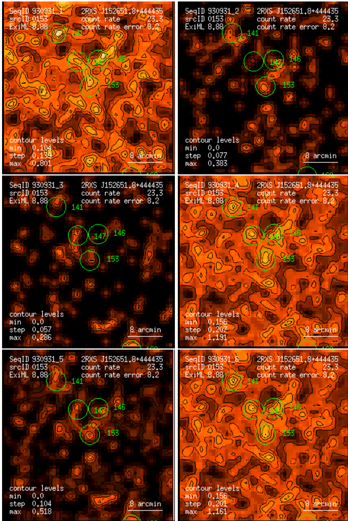
Figure 153: RASS 930931: detection 0153: band rate images, Gaussian filter: (1) PSPC channels 11 – 41, (2) 52 – 90, (3) 91 – 201, (4) 11 – 235, (5) 52 – 201, (6) 11 – 201. Broad band rates in counts/ks. Band rate contour levels in counts/ks/arcmin 2 .
