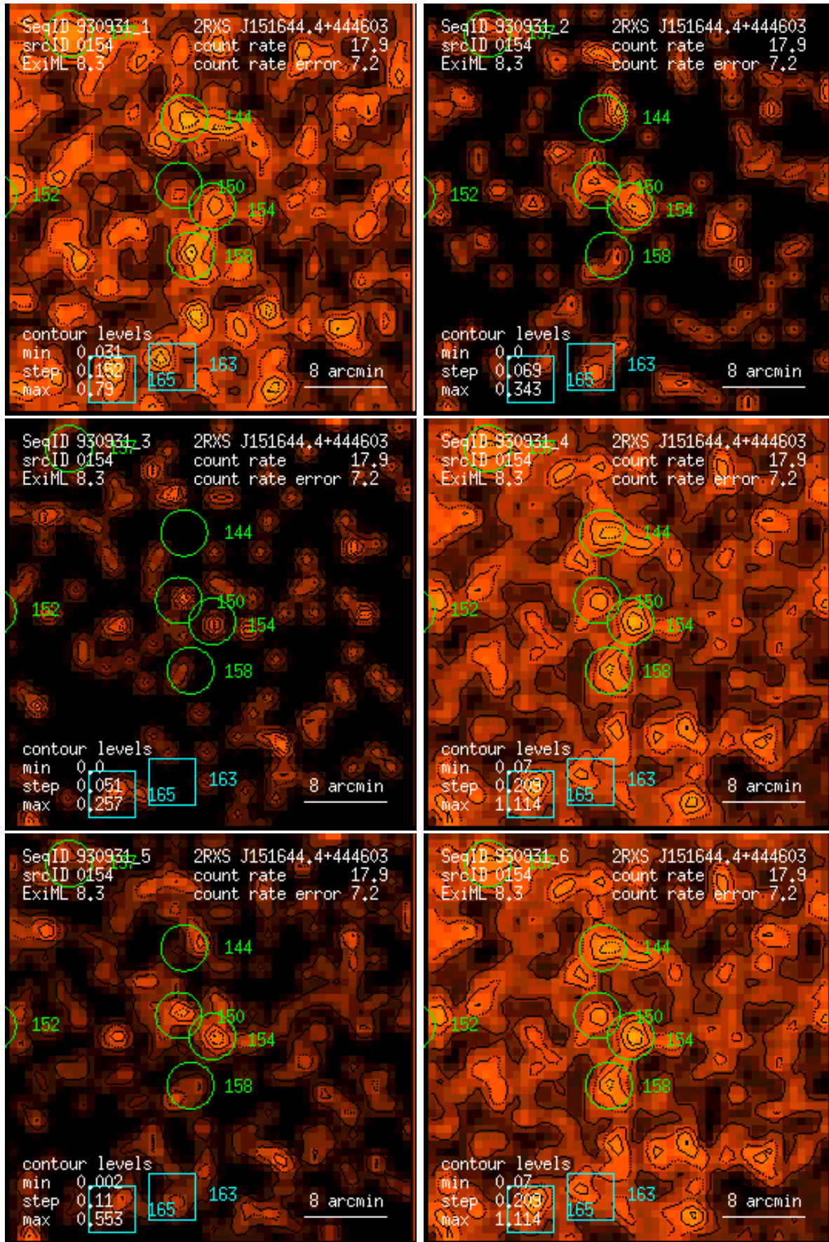
Figure 154: RASS 930931: detection 0154: band rate images, Gaussian filter: (1) PSPC channels 11 – 41, (2) 52 – 90, (3) 91 – 201, (4) 11 – 235, (5) 52 – 201, (6) 11 – 201. Broad band rates in counts/ks. Band rate contour levels in counts/ks/arcmin 2 .
