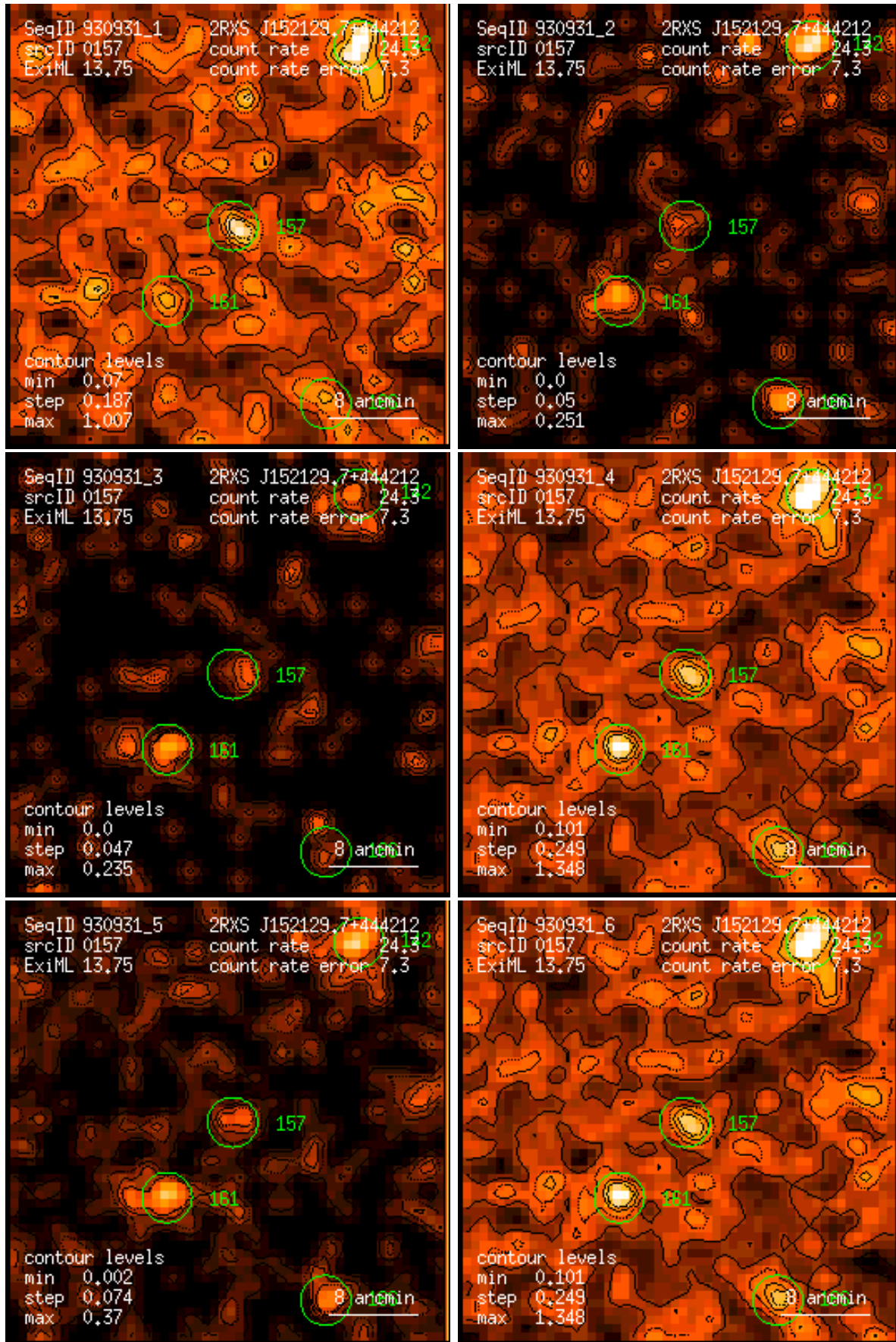
Figure 157: RASS 930931: detection 0157: band rate images, Gaussian filter: (1) PSPC channels 11 – 41, (2) 52 – 90, (3) 91 – 201, (4) 11 – 235, (5) 52 – 201, (6) 11 – 201. Broad band rates in counts/ks. Band rate contour levels in counts/ks/arcmin 2 .
