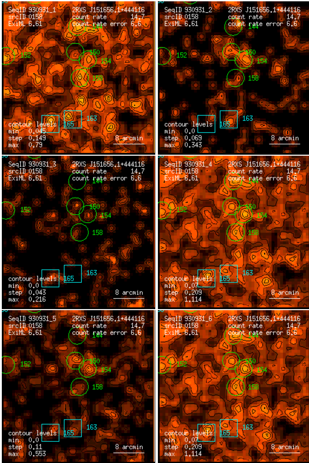
Figure 158: RASS 930931: detection 0158: band rate images, Gaussian filter: (1) PSPC channels 11 – 41, (2) 52 – 90, (3) 91 – 201, (4) 11 – 235, (5) 52 – 201, (6) 11 – 201. Broad band rates in counts/ks. Band rate contour levels in counts/ks/arcmin 2 .
