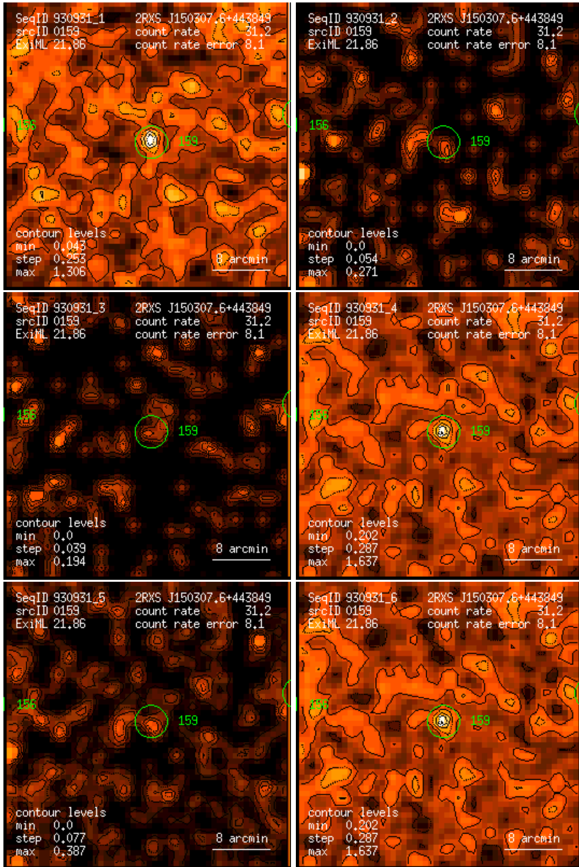
Figure 159: RASS 930931: detection 0159: band rate images, Gaussian filter: (1) PSPC channels 11 – 41, (2) 52 – 90, (3) 91 – 201, (4) 11 – 235, (5) 52 – 201, (6) 11 – 201. Broad band rates in counts/ks. Band rate contour levels in counts/ks/arcmin 2 .
