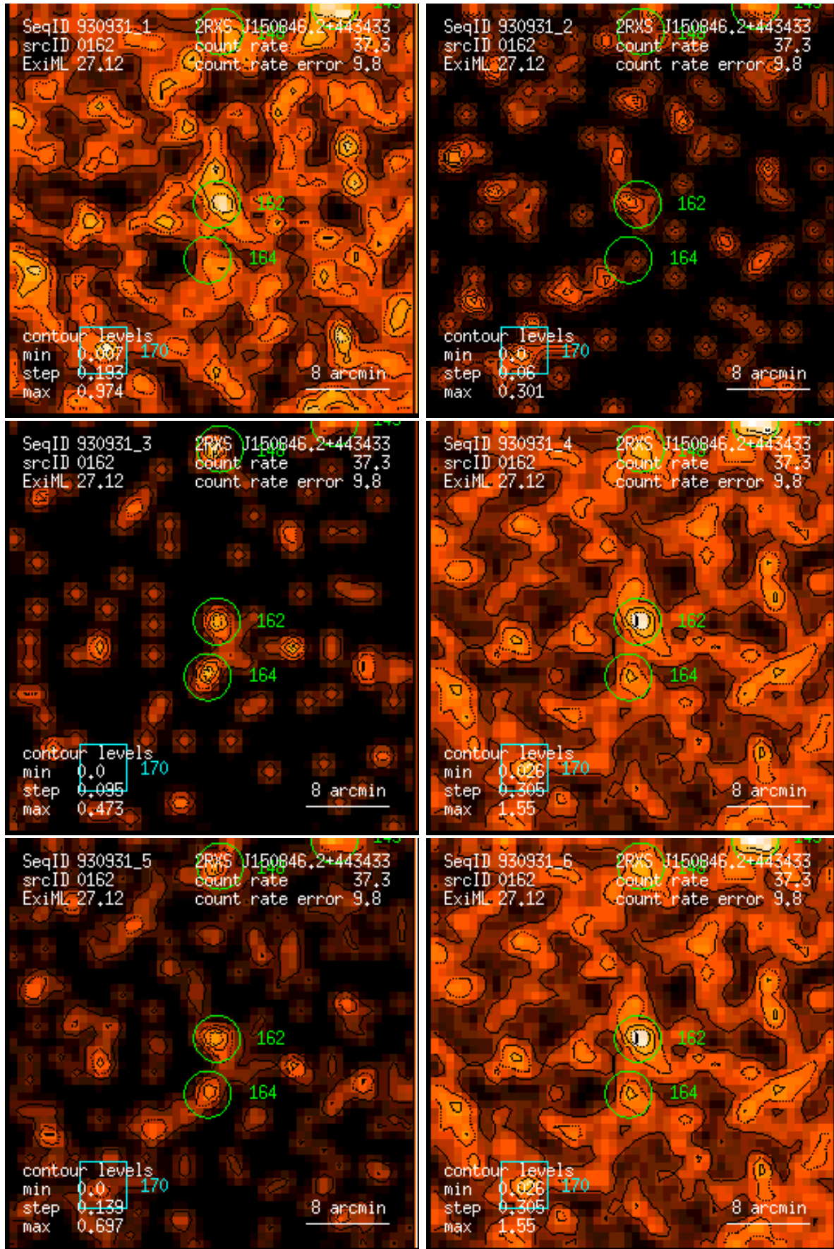
Figure 162: RASS 930931: detection 0162: band rate images, Gaussian filter: (1) PSPC channels 11 – 41, (2) 52 – 90, (3) 91 – 201, (4) 11 – 235, (5) 52 – 201, (6) 11 – 201. Broad band rates in counts/ks. Band rate contour levels in counts/ks/arcmin 2 .
