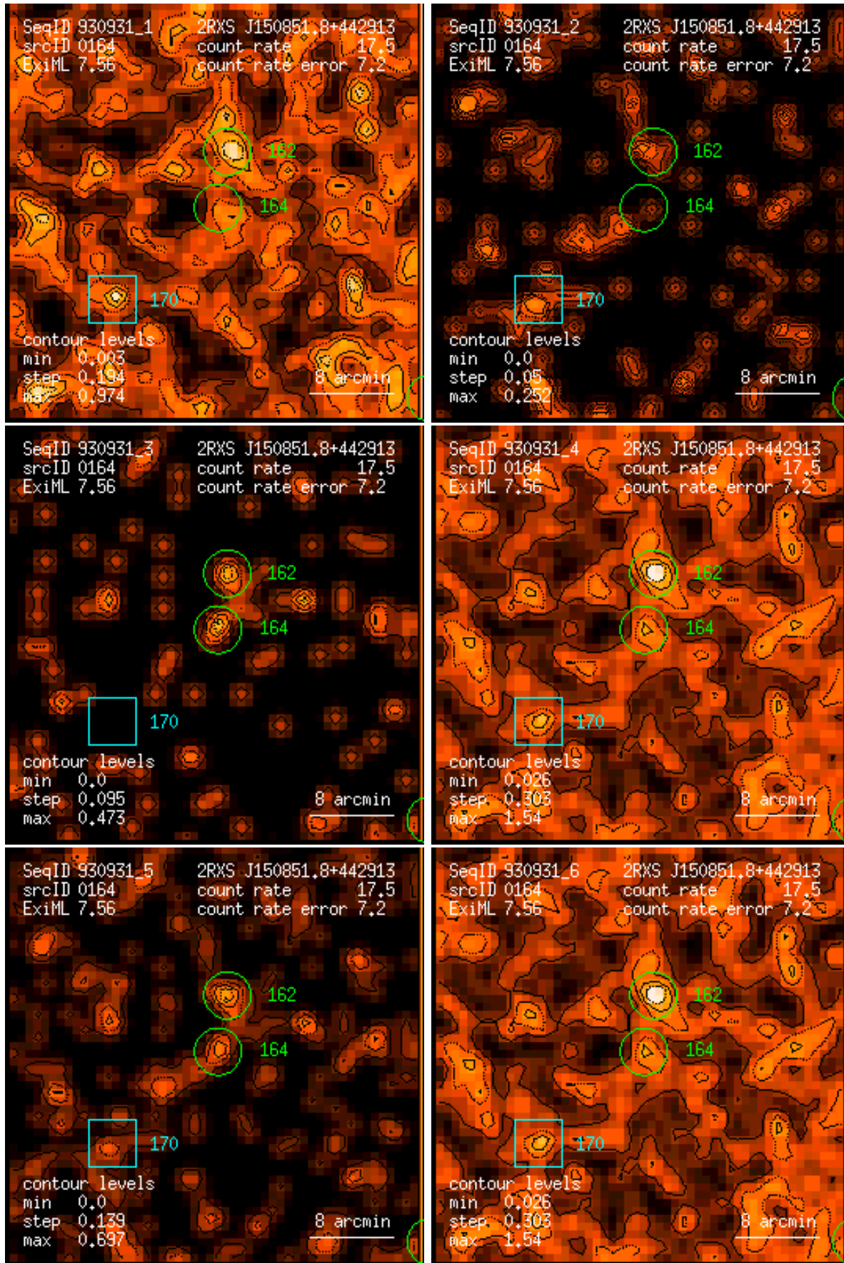
Figure 164: RASS 930931: detection 0164: band rate images, Gaussian filter: (1) PSPC channels 11 – 41, (2) 52 – 90, (3) 91 – 201, (4) 11 – 235, (5) 52 – 201, (6) 11 – 201. Broad band rates in counts/ks. Band rate contour levels in counts/ks/arcmin 2 .
