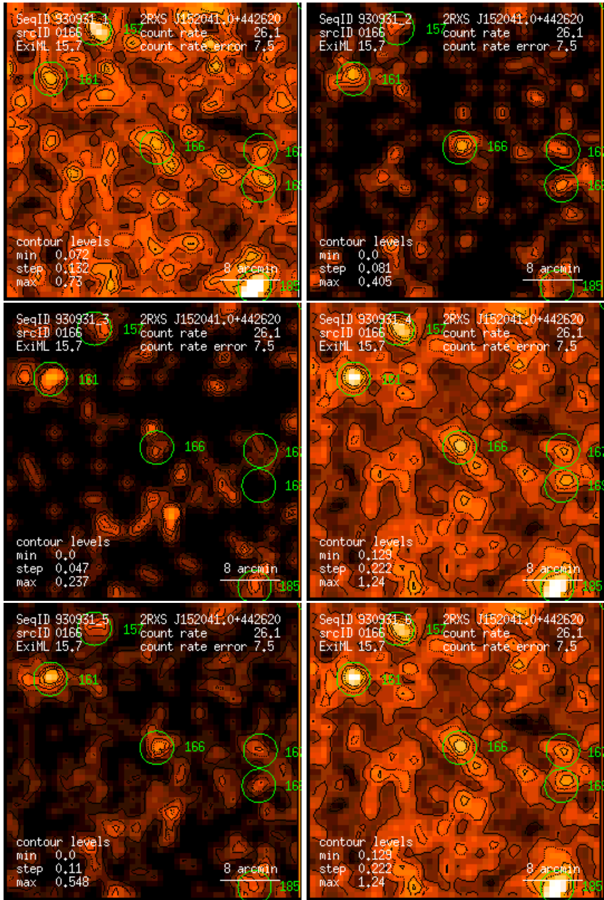
Figure 166: RASS 930931: detection 0166: band rate images, Gaussian filter: (1) PSPC channels 11 – 41, (2) 52 – 90, (3) 91 – 201, (4) 11 – 235, (5) 52 – 201, (6) 11 – 201. Broad band rates in counts/ks. Band rate contour levels in counts/ks/arcmin 2 .
