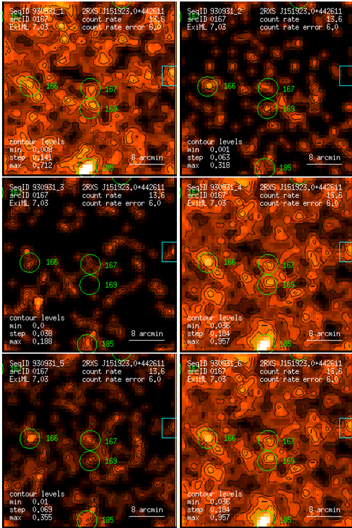
Figure 167: RASS 930931: detection 0167: band rate images, Gaussian filter: (1) PSPC channels 11 – 41, (2) 52 – 90, (3) 91 – 201, (4) 11 – 235, (5) 52 – 201, (6) 11 – 201. Broad band rates in counts/ks. Band rate contour levels in counts/ks/arcmin 2 .
