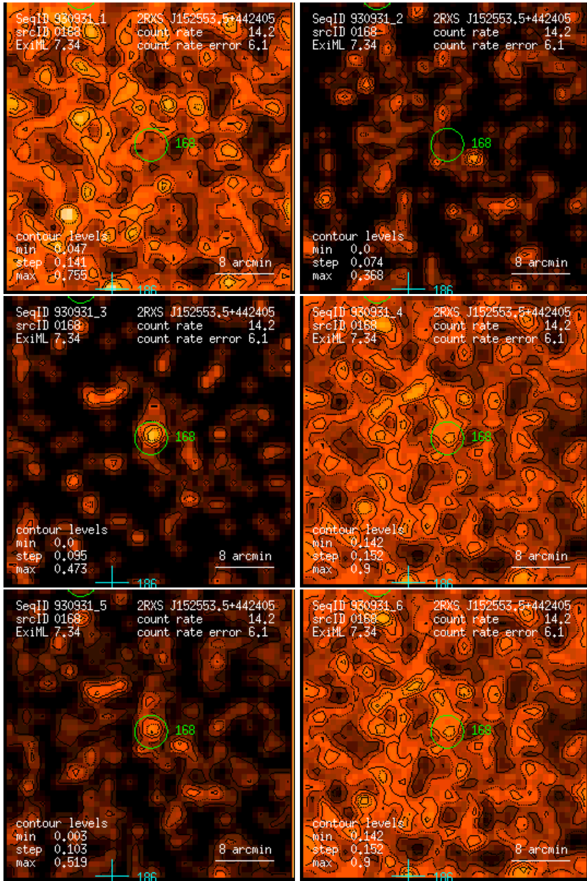
Figure 168: RASS 930931: detection 0168: band rate images, Gaussian filter: (1) PSPC channels 11 – 41, (2) 52 – 90, (3) 91 – 201, (4) 11 – 235, (5) 52 – 201, (6) 11 – 201. Broad band rates in counts/ks. Band rate contour levels in counts/ks/arcmin 2 .
