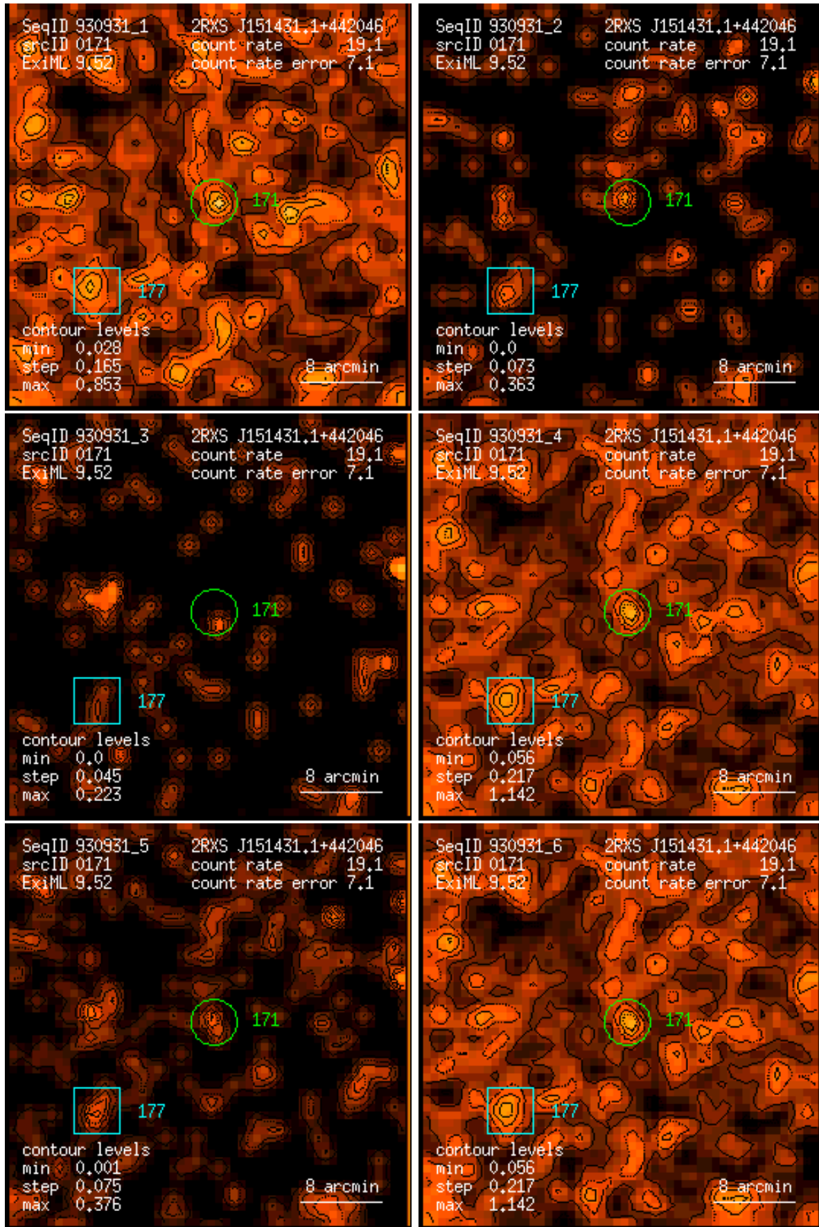
Figure 171: RASS 930931: detection 0171: band rate images, Gaussian filter: (1) PSPC channels 11 – 41, (2) 52 – 90, (3) 91 – 201, (4) 11 – 235, (5) 52 – 201, (6) 11 – 201. Broad band rates in counts/ks. Band rate contour levels in counts/ks/arcmin 2 .
