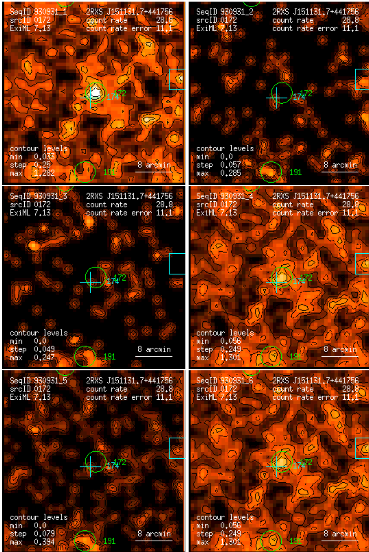
Figure 172: RASS 930931: detection 0172: band rate images, Gaussian filter: (1) PSPC channels 11 – 41, (2) 52 – 90, (3) 91 – 201, (4) 11 – 235, (5) 52 – 201, (6) 11 – 201. Broad band rates in counts/ks. Band rate contour levels in counts/ks/arcmin 2 .
