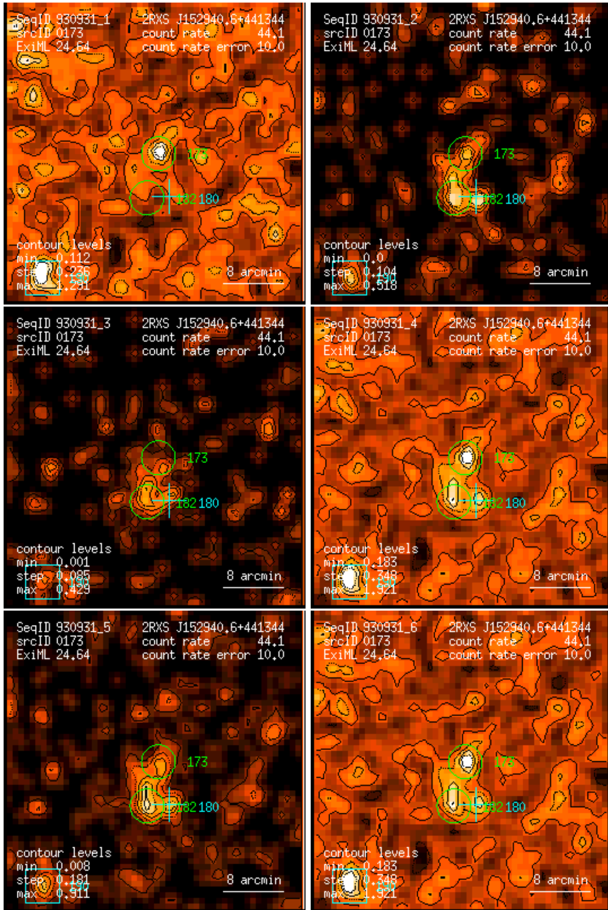
Figure 173: RASS 930931: detection 0173: band rate images, Gaussian filter: (1) PSPC channels 11 – 41, (2) 52 – 90, (3) 91 – 201, (4) 11 – 235, (5) 52 – 201, (6) 11 – 201. Broad band rates in counts/ks. Band rate contour levels in counts/ks/arcmin 2 .
