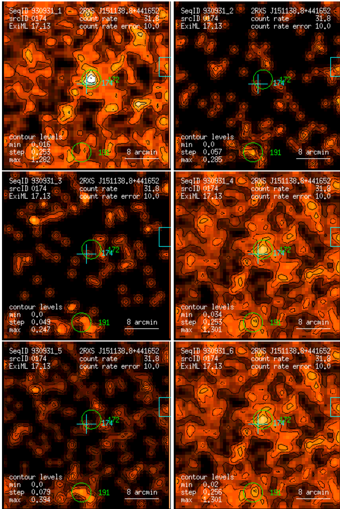
Figure 174: RASS 930931: detection 0174: band rate images, Gaussian filter: (1) PSPC channels 11 – 41, (2) 52 – 90, (3) 91 – 201, (4) 11 – 235, (5) 52 – 201, (6) 11 – 201. Broad band rates in counts/ks. Band rate contour levels in counts/ks/arcmin 2 .
