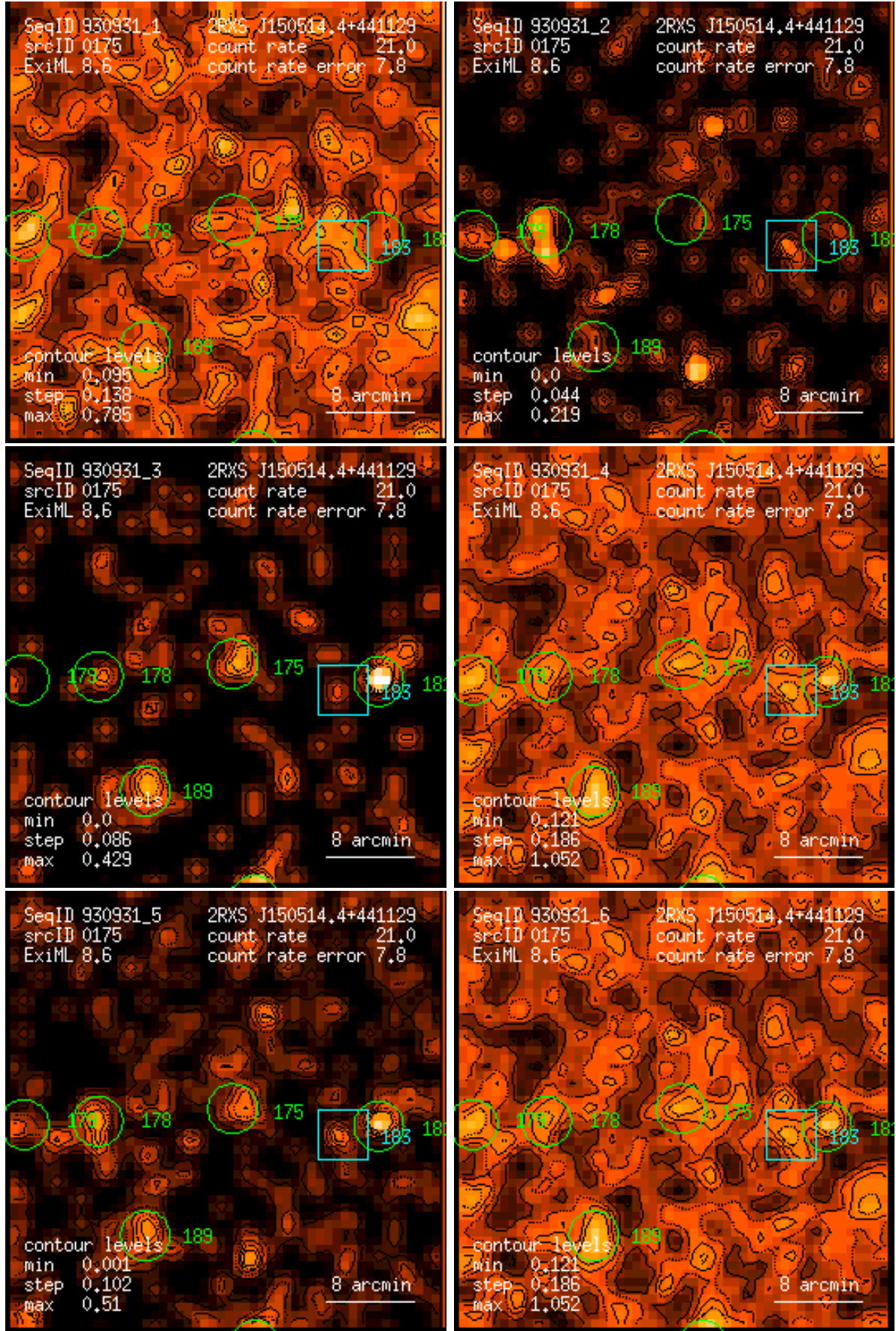
Figure 175: RASS 930931: detection 0175: band rate images, Gaussian filter: (1) PSPC channels 11 – 41, (2) 52 – 90, (3) 91 – 201, (4) 11 – 235, (5) 52 – 201, (6) 11 – 201. Broad band rates in counts/ks. Band rate contour levels in counts/ks/arcmin 2 .
