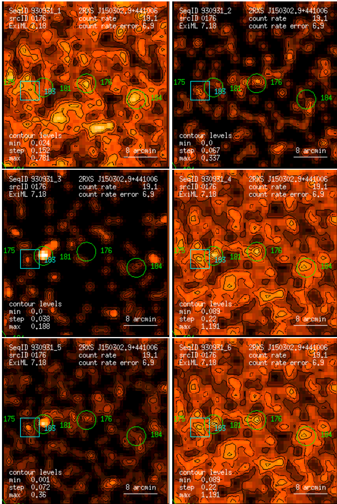
Figure 176: RASS 930931: detection 0176: band rate images, Gaussian filter: (1) PSPC channels 11 – 41, (2) 52 – 90, (3) 91 – 201, (4) 11 – 235, (5) 52 – 201, (6) 11 – 201. Broad band rates in counts/ks. Band rate contour levels in counts/ks/arcmin 2 .
