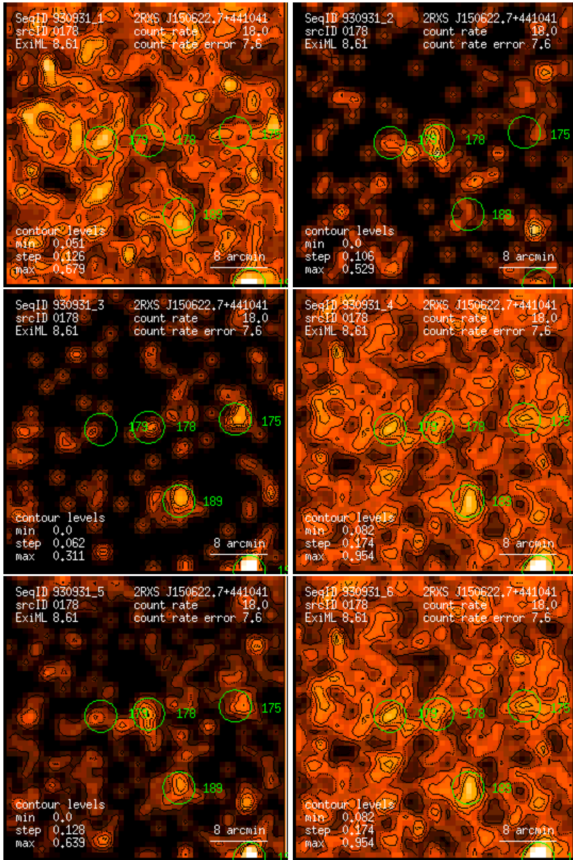
Figure 178: RASS 930931: detection 0178: band rate images, Gaussian filter: (1) PSPC channels 11 – 41, (2) 52 – 90, (3) 91 – 201, (4) 11 – 235, (5) 52 – 201, (6) 11 – 201. Broad band rates in counts/ks. Band rate contour levels in counts/ks/arcmin 2 .
