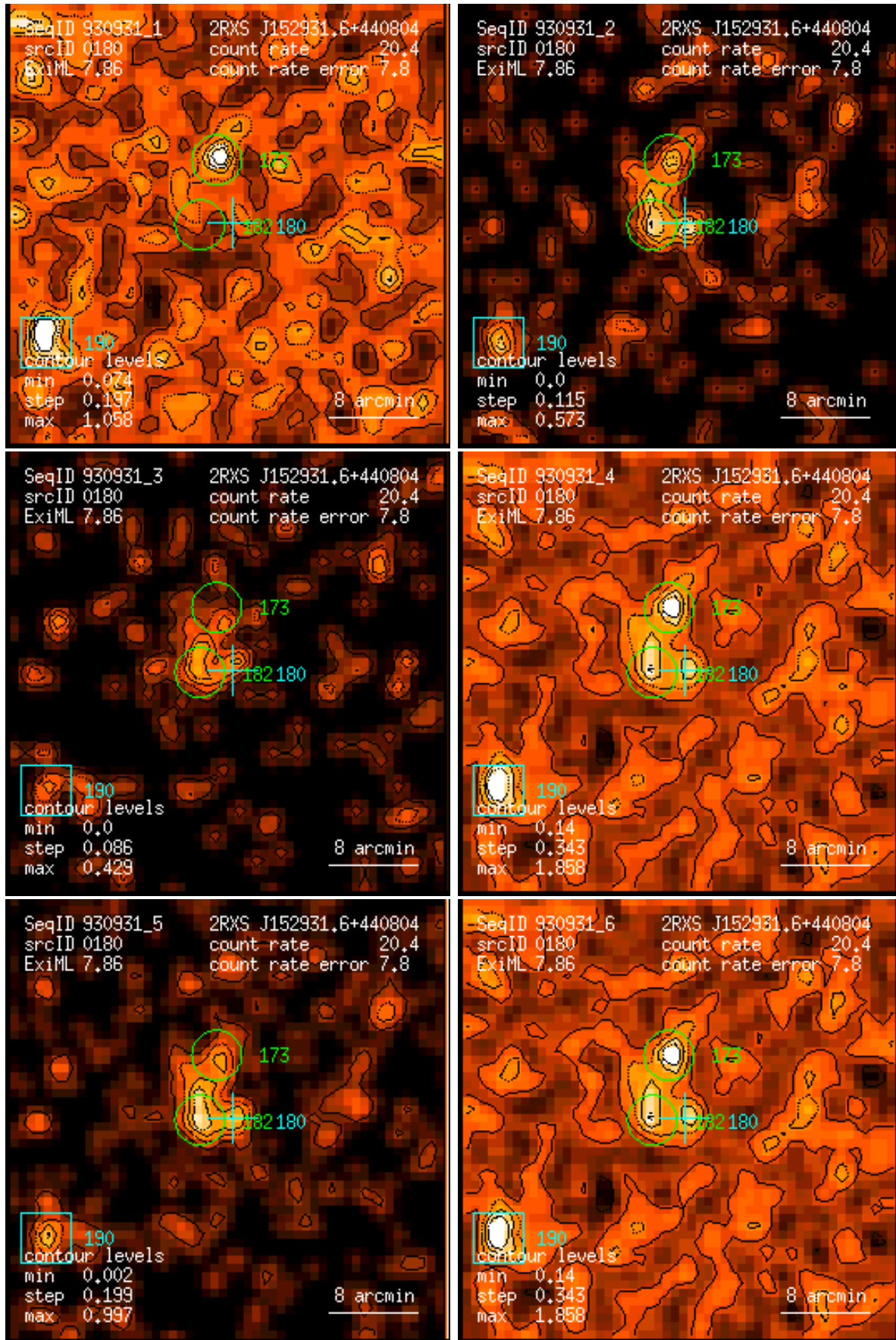
Figure 180: RASS 930931: detection 0180: band rate images, Gaussian filter: (1) PSPC channels 11 – 41, (2) 52 – 90, (3) 91 – 201, (4) 11 – 235, (5) 52 – 201, (6) 11 – 201. Broad band rates in counts/ks. Band rate contour levels in counts/ks/arcmin 2 .
