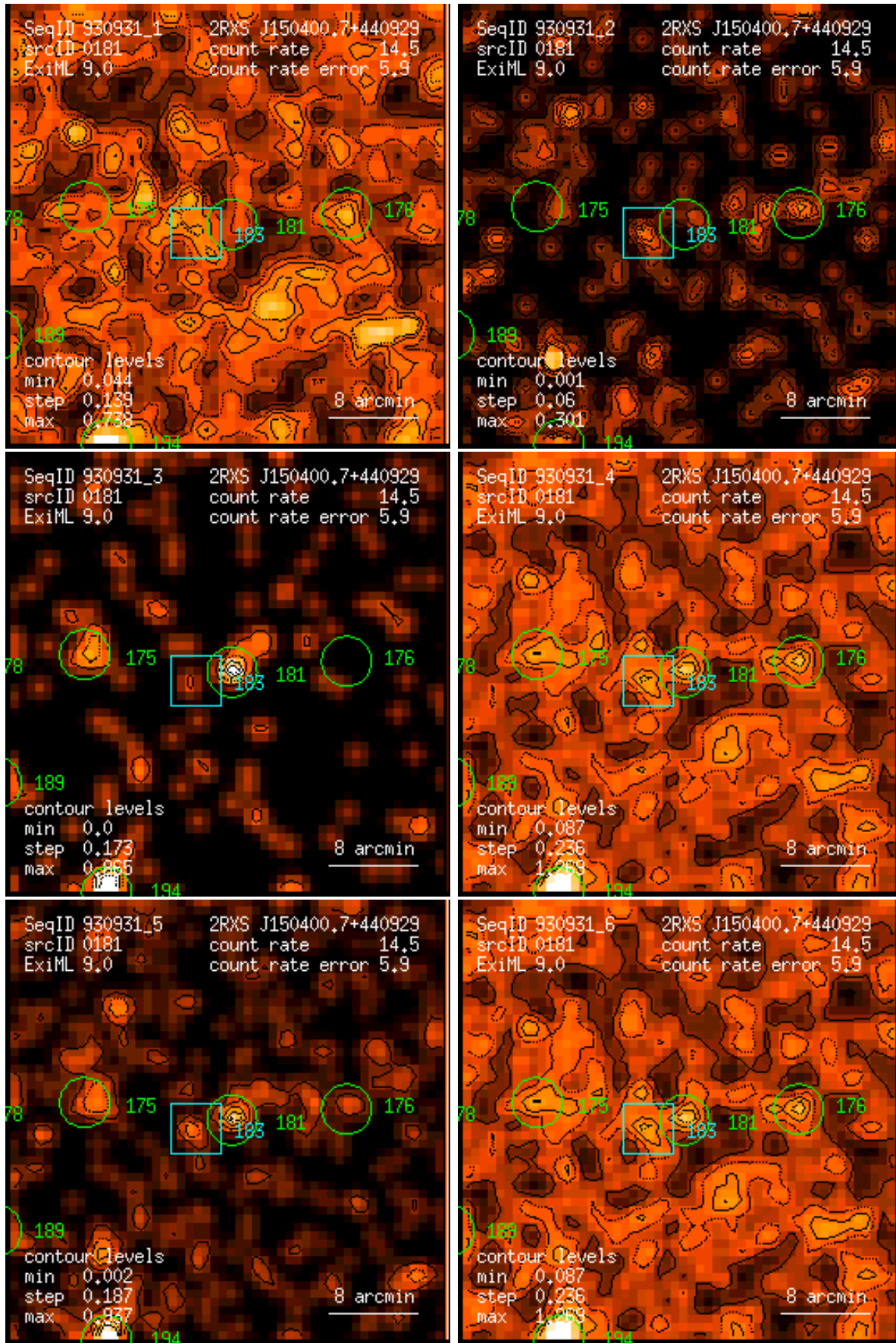
Figure 181: RASS 930931: detection 0181: band rate images, Gaussian filter: (1) PSPC channels 11 – 41, (2) 52 – 90, (3) 91 – 201, (4) 11 – 235, (5) 52 – 201, (6) 11 – 201. Broad band rates in counts/ks. Band rate contour levels in counts/ks/arcmin 2 .
